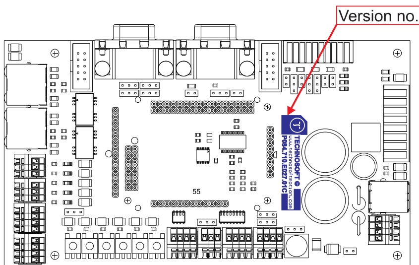
Figure 2.4.1. IO-iPOS4808MY V0.1C board version identification
