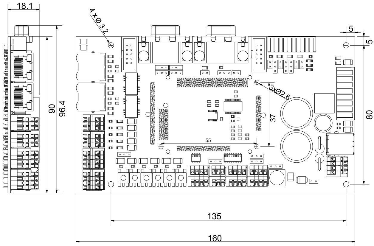
Figure 2.3.1. IO-iPOS4808MY board dimensions
