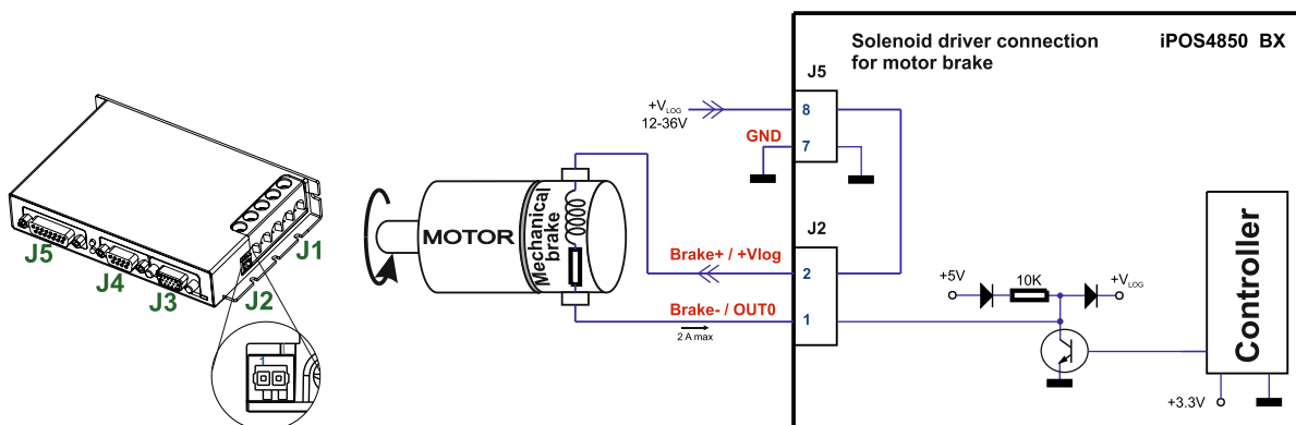
Figure 0.6. 24V Digital NPN Outputs connection
