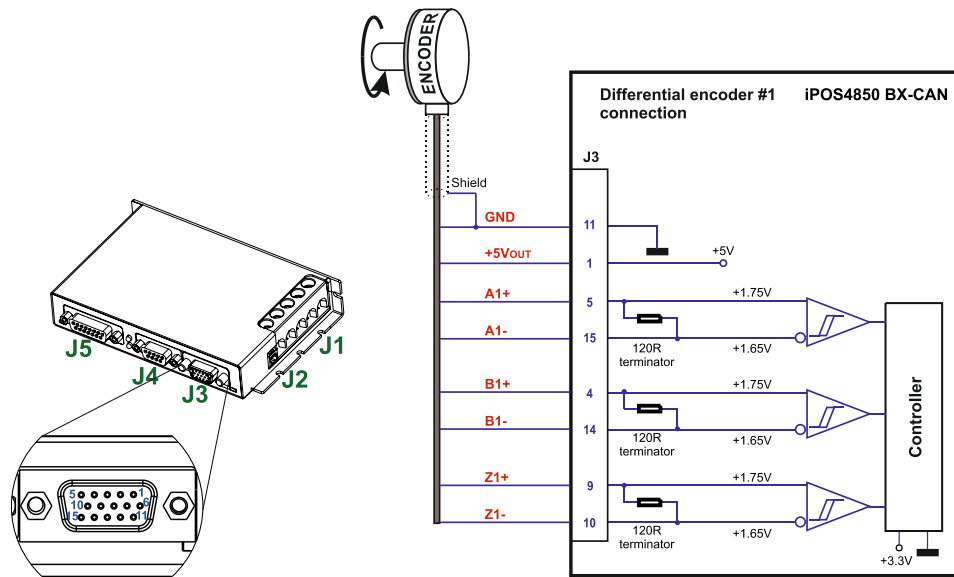
Figure 0.11. Differential incremental encoder #1 connection
