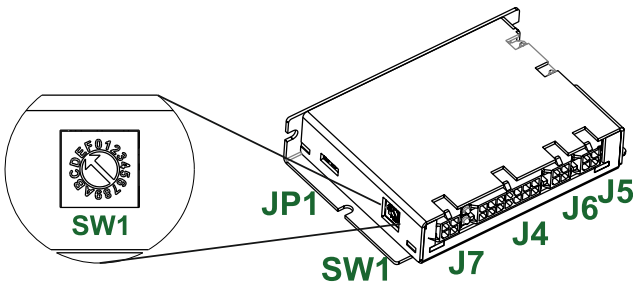
Figure 3.30. SW1 Location
