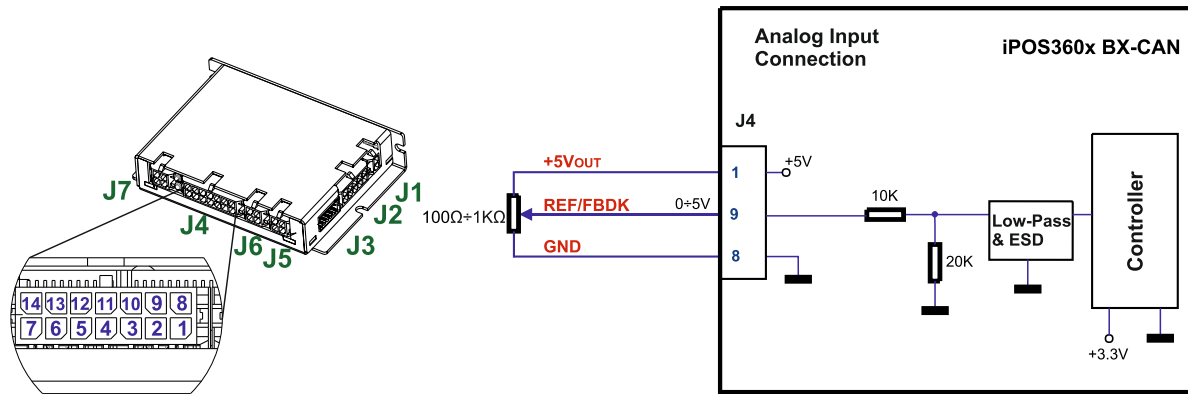
Figure 3.11. 0-5V Analog inputs connection
