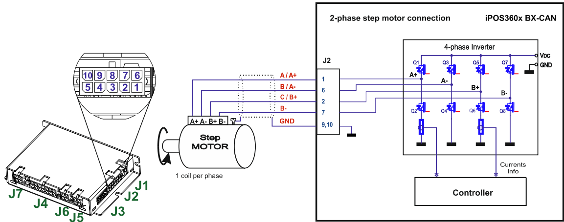
Figure 3.14. 2-phase step motor connection, one coil per phase
