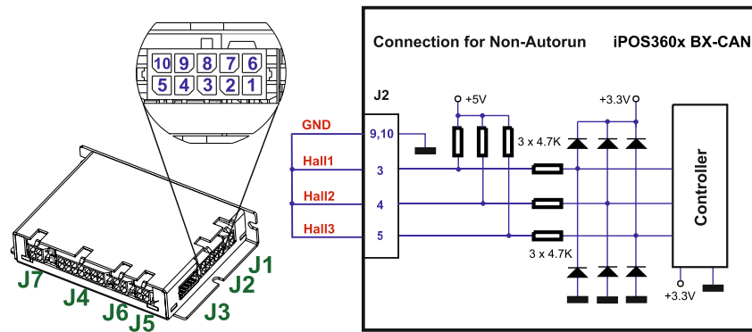
Figure 3.28. Temporary connection during power-on to disable the drive from Autorun mode
