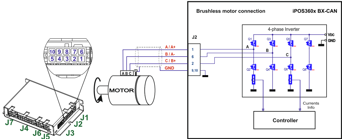
Figure 3.13. Brushless motor connection
