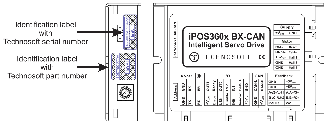
Figure 2.3.1. iPOS360X BX-CAN identification labels
