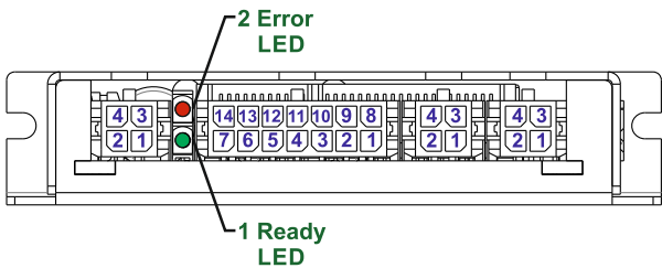
Figure 3.31. LED indicators
