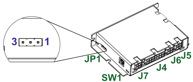
Figure 3.29. JP1 Location
