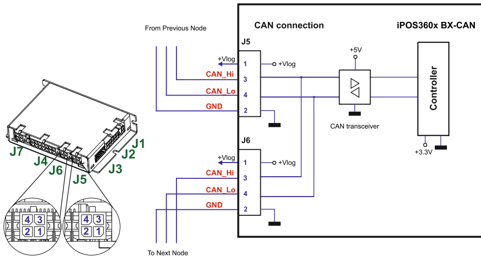
Figure 3.26. CAN connection
