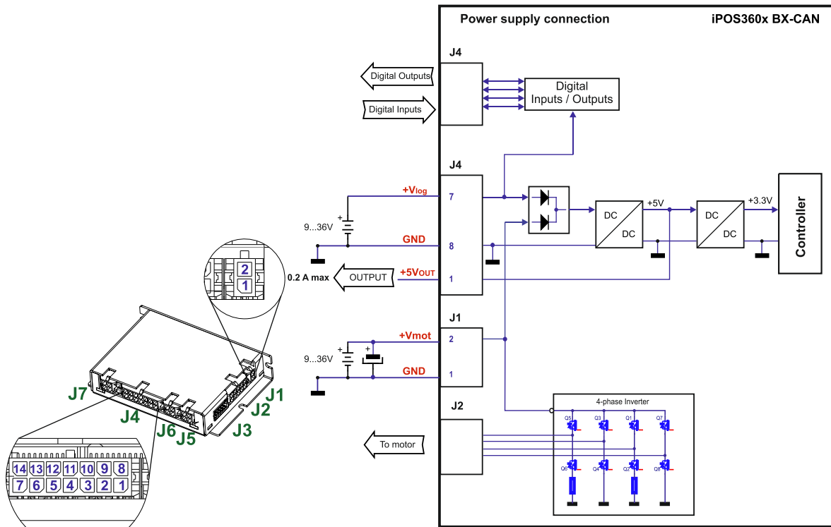
Figure 3.24. Supply connection
