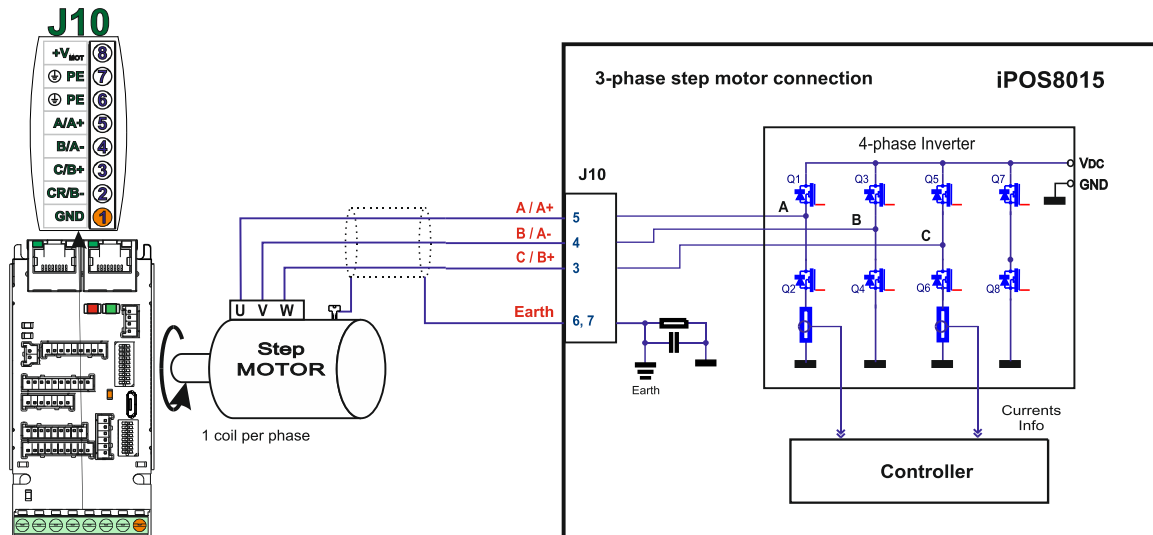
Figure 16. 3-phase step motor connection
