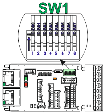
Figure 40. SW1 – DIP Switch settings
