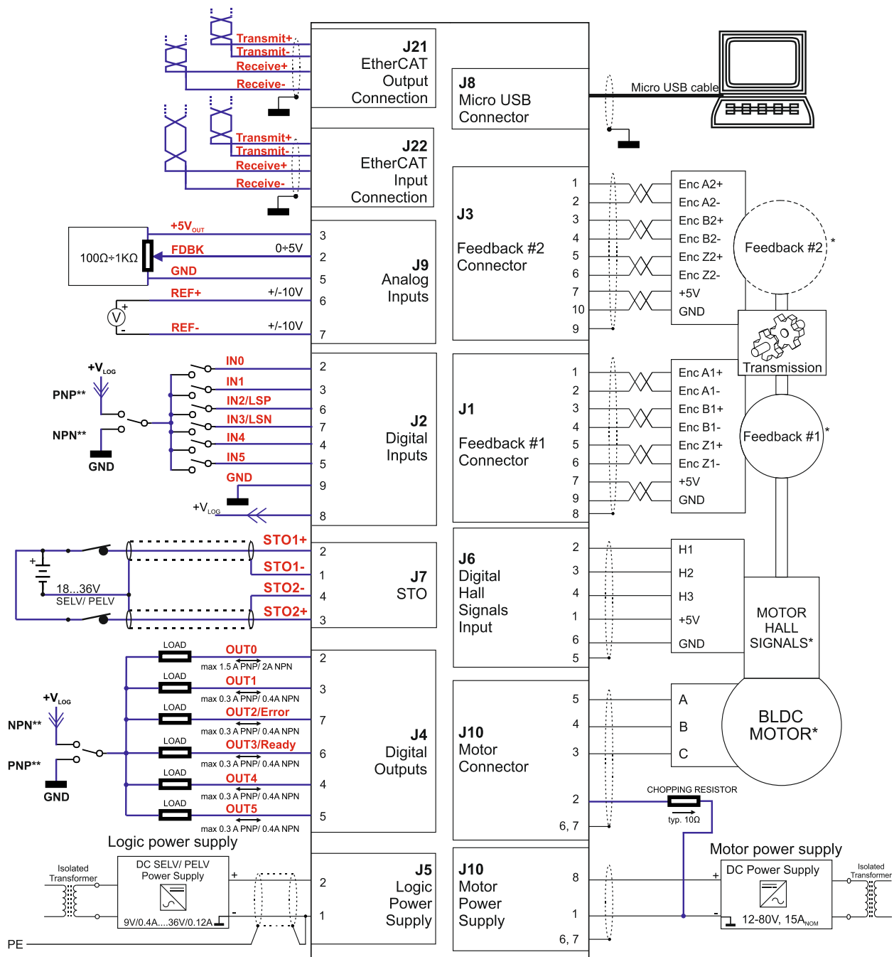
Figure 4. iPOS8015 XZ-CAT Connection diagram
