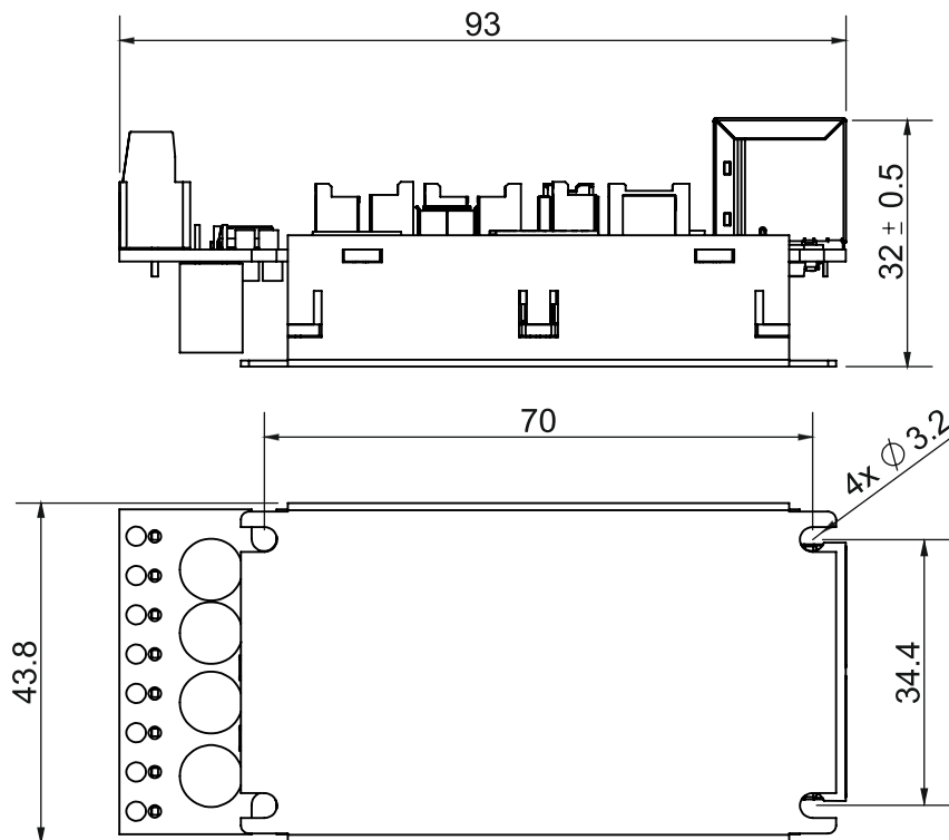
Figure 2. iPOS8015 XZ-CAT drive dimensions
