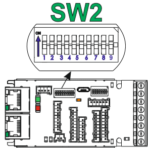
Figure 25. SW2 DIP Switch
