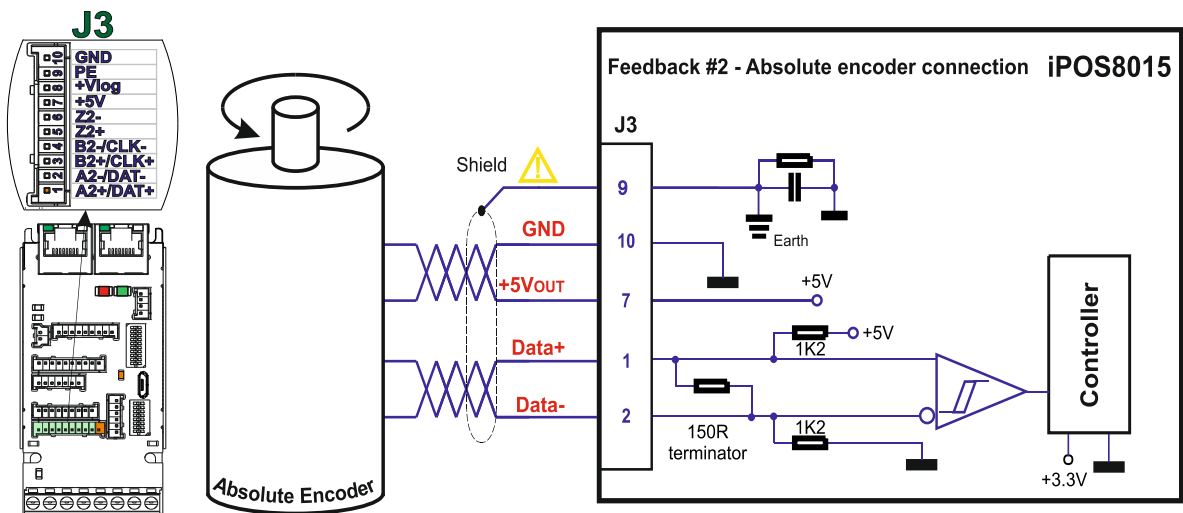
Figure 23. Absolute encoder #2 connection: Nikon, Panasonic, Sanyo Denki, Tamagawa
