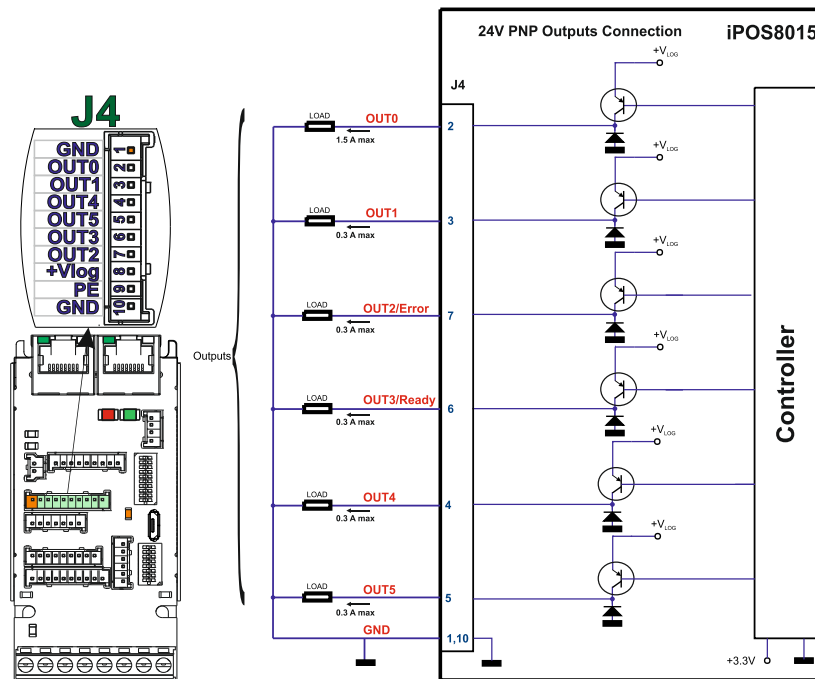
Figure 8. 24V Digital PNP Outputs connection
