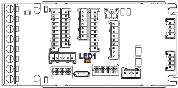
Figure 39. LED indicators
