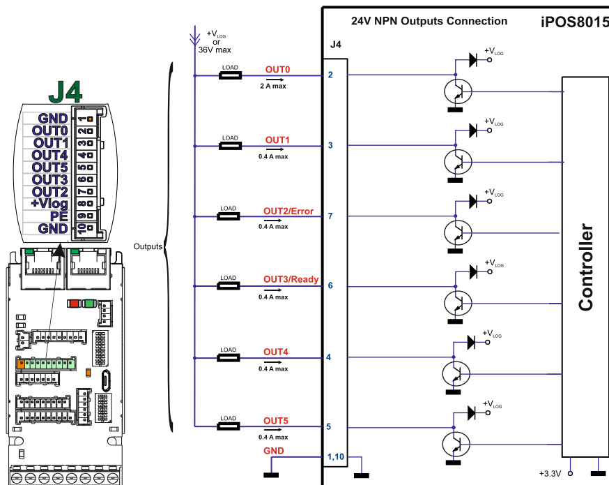
Figure 9. 24V Digital NPN Outputs connection
