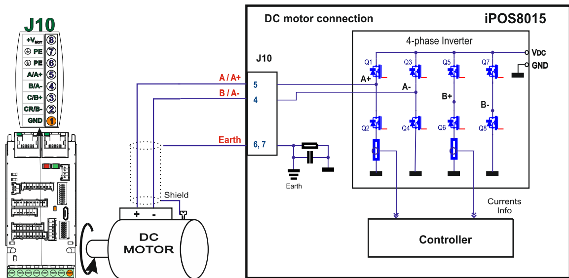
Figure 17. DC Motor connection
