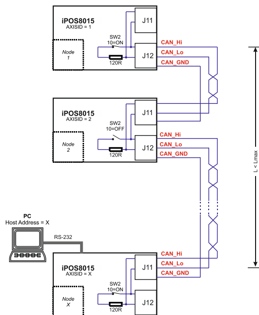
Figure 34. Multiple-Axis CAN network
