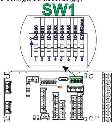
Figure 38. SW1 – DIP Switch settings
