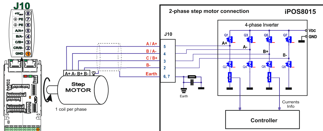
Figure 14. 2-phase step motor connection, one coil per phase
