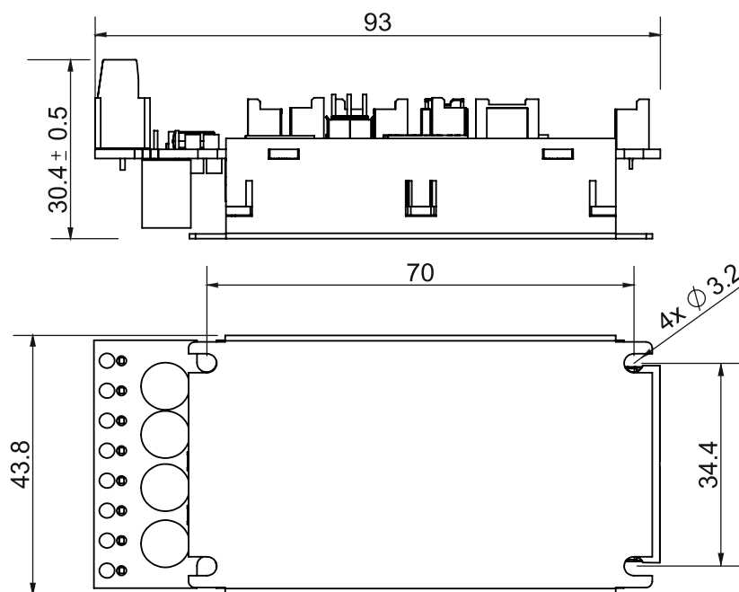
Figure 3. iPOS8015 XZ-CAN drive dimensions
