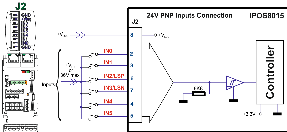
Figure 6. 24V Digital PNP Inputs connection
