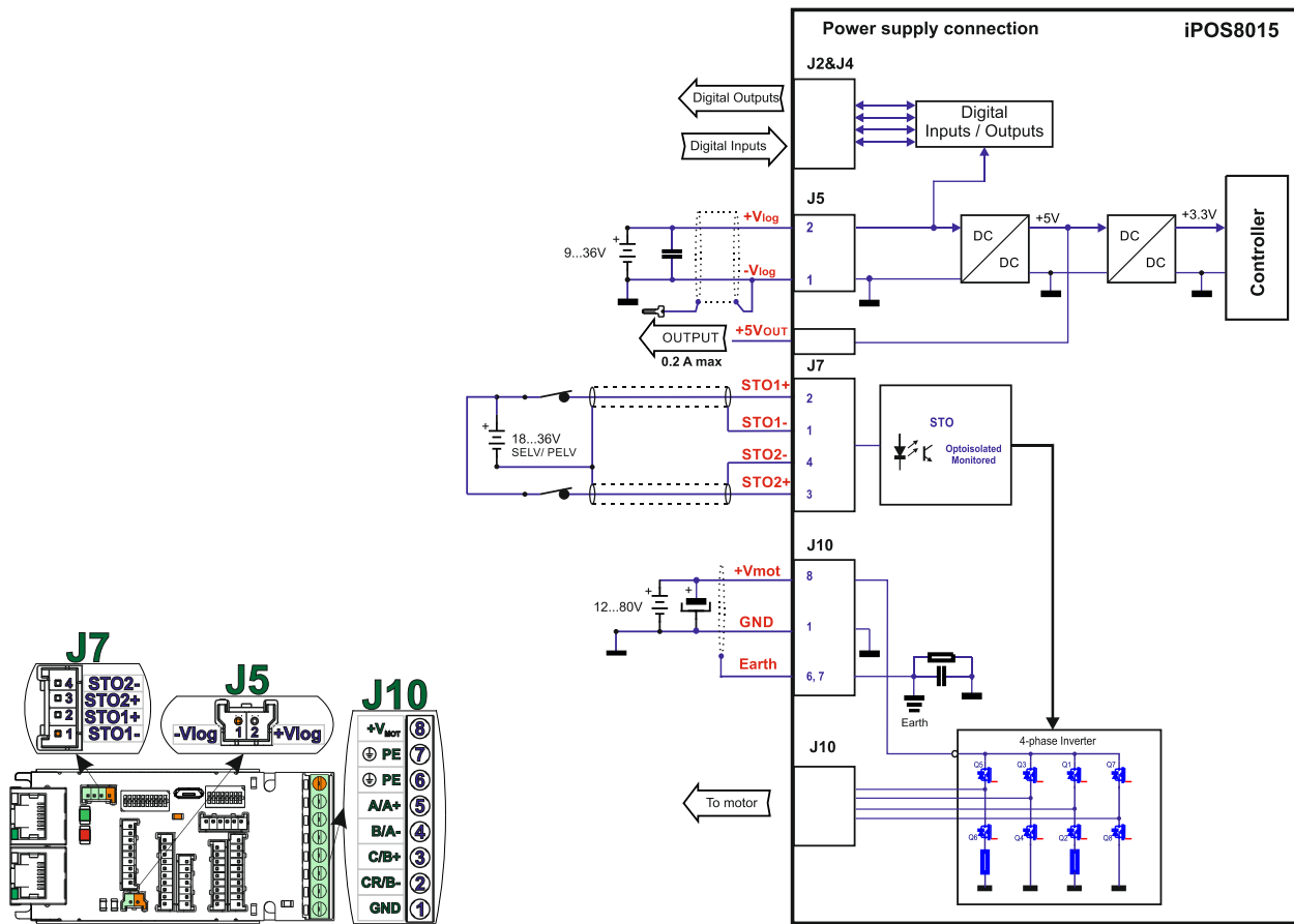
Figure 29. Supply connection
