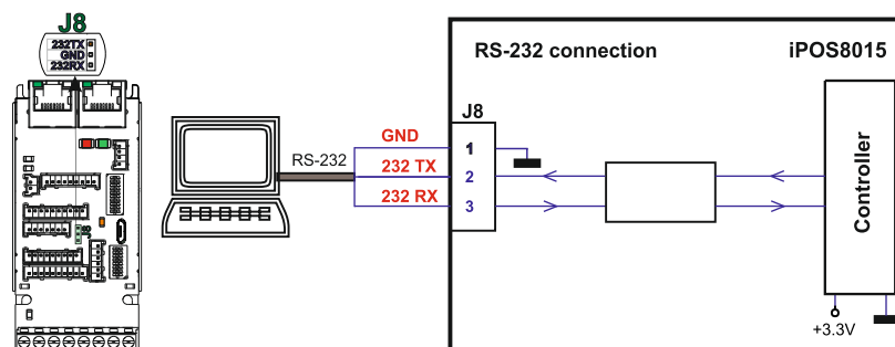
Figure 3.32. Low level TTL connection
