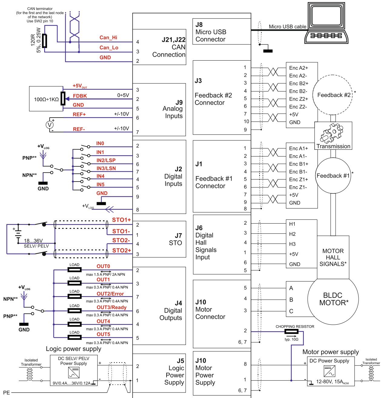
Figure 5. iPOS8015 XZ-CAN Connection diagram
