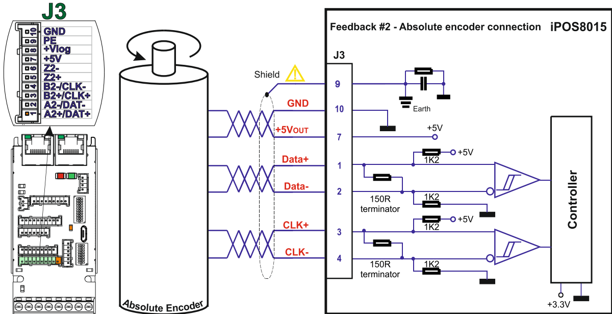
Figure 22. Absolute encoder #2 connection: SSI, BISS-C, EnDAT
