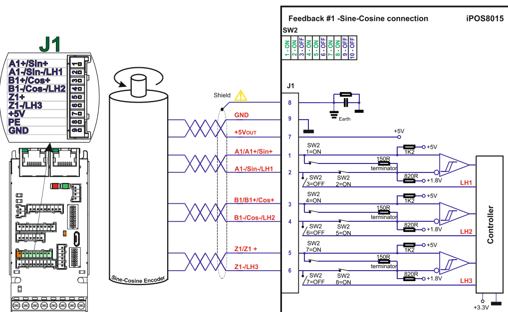
Figure 21. Sine-Cosine analogue encoder connection
