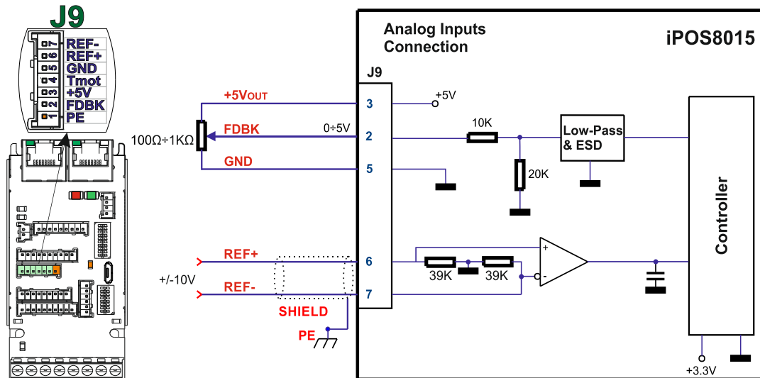
Figure 12. 0-5V Analog inputs connection
