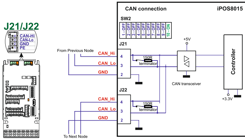
Figure 33. CAN connection
