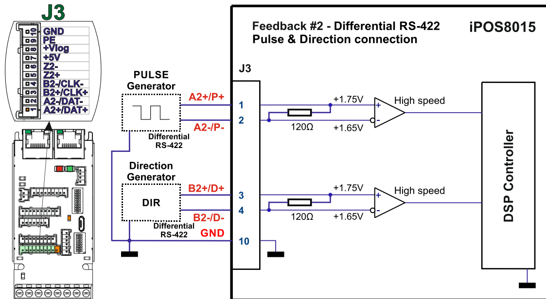
Figure 28. Digital Hall connection for Motor + Hall control
