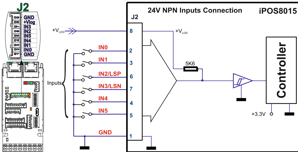
Figure 7. 24V Digital NPN Inputs connection
