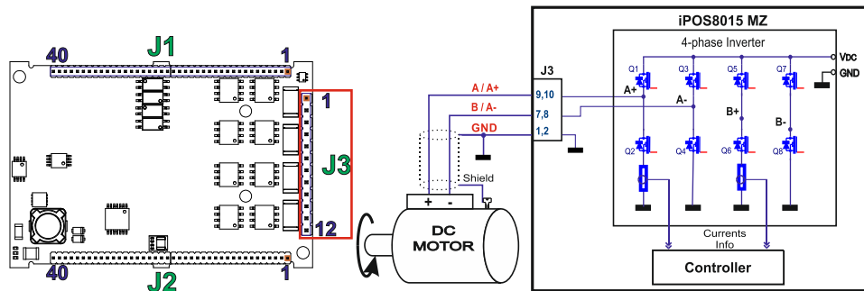
Figure 13.16. DC Motor connection
