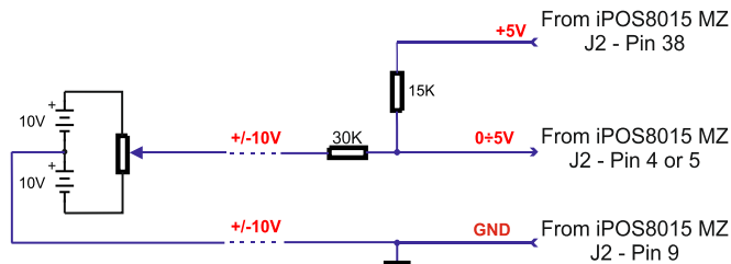
Figure 13.9. \pm 10 V to 0-5V adapter
