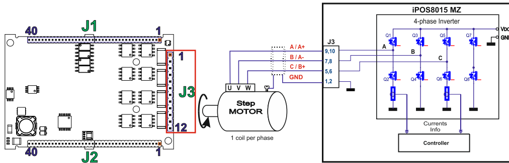
Figure 13.15. 3-phase step motor connection
