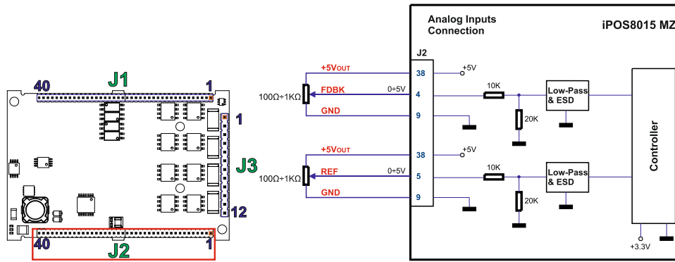
Figure 13.8. 0-5V Analog inputs connection
