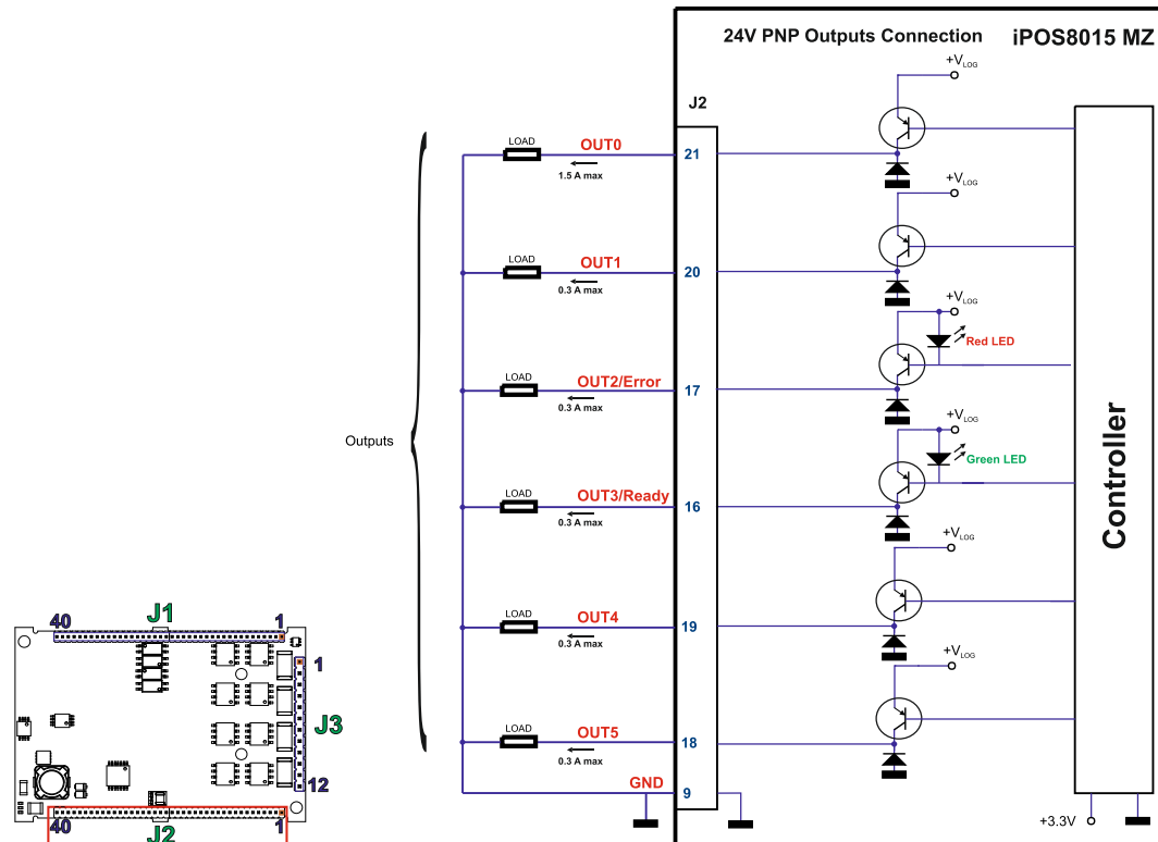
Figure 13.5. 24V Digital PNP Outputs connection
