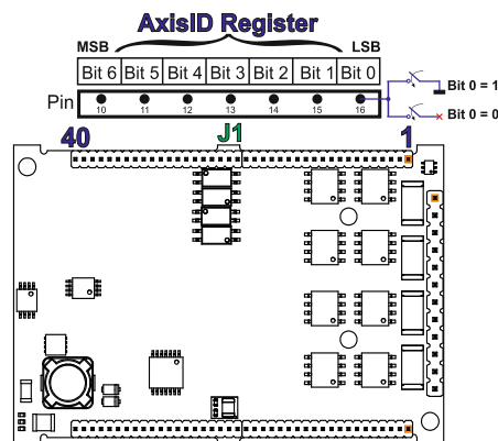
Figure 13.34. J1 – Axis ID pins for CAN drives
