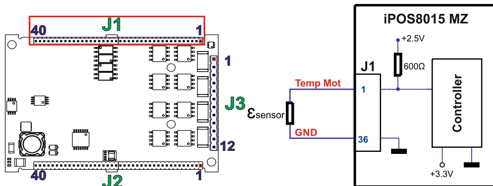
Figure 13.7. Temperature sensor connection
