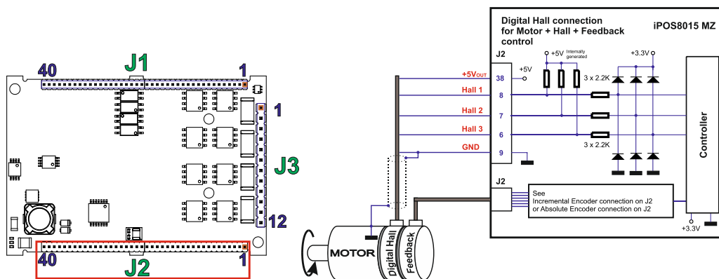
Figure 13.24. Digital Hall connection
