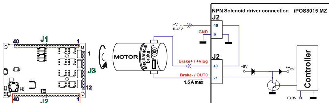
Figure 10 Solenoid driver connection
