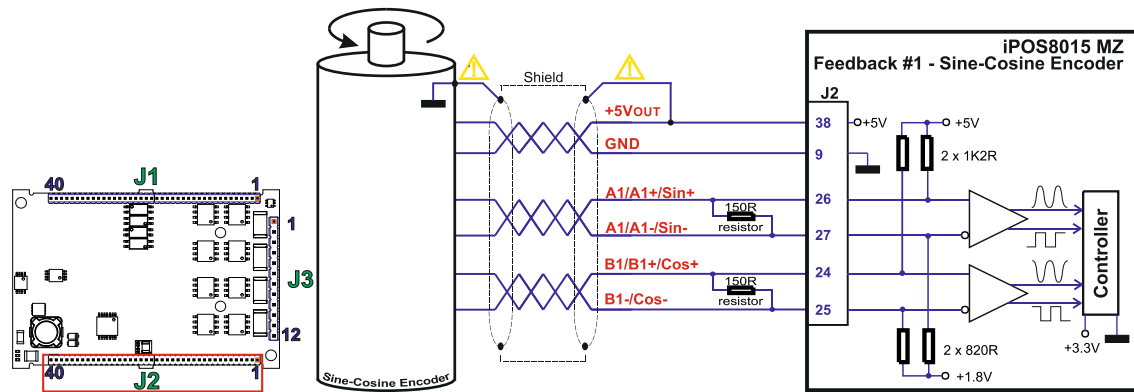
Figure 13.20. Sine-Cosine analogue encoder connection
