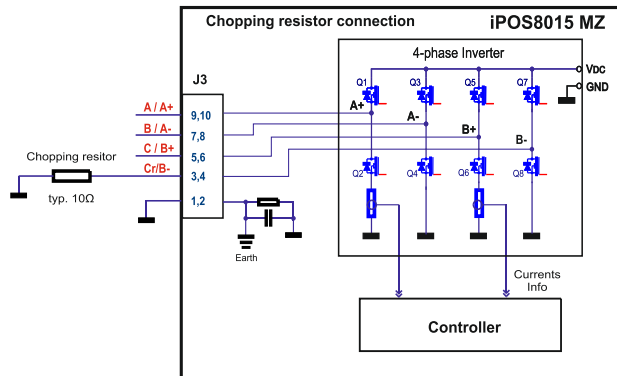
Figure 13.27. Chopping resistor connection
