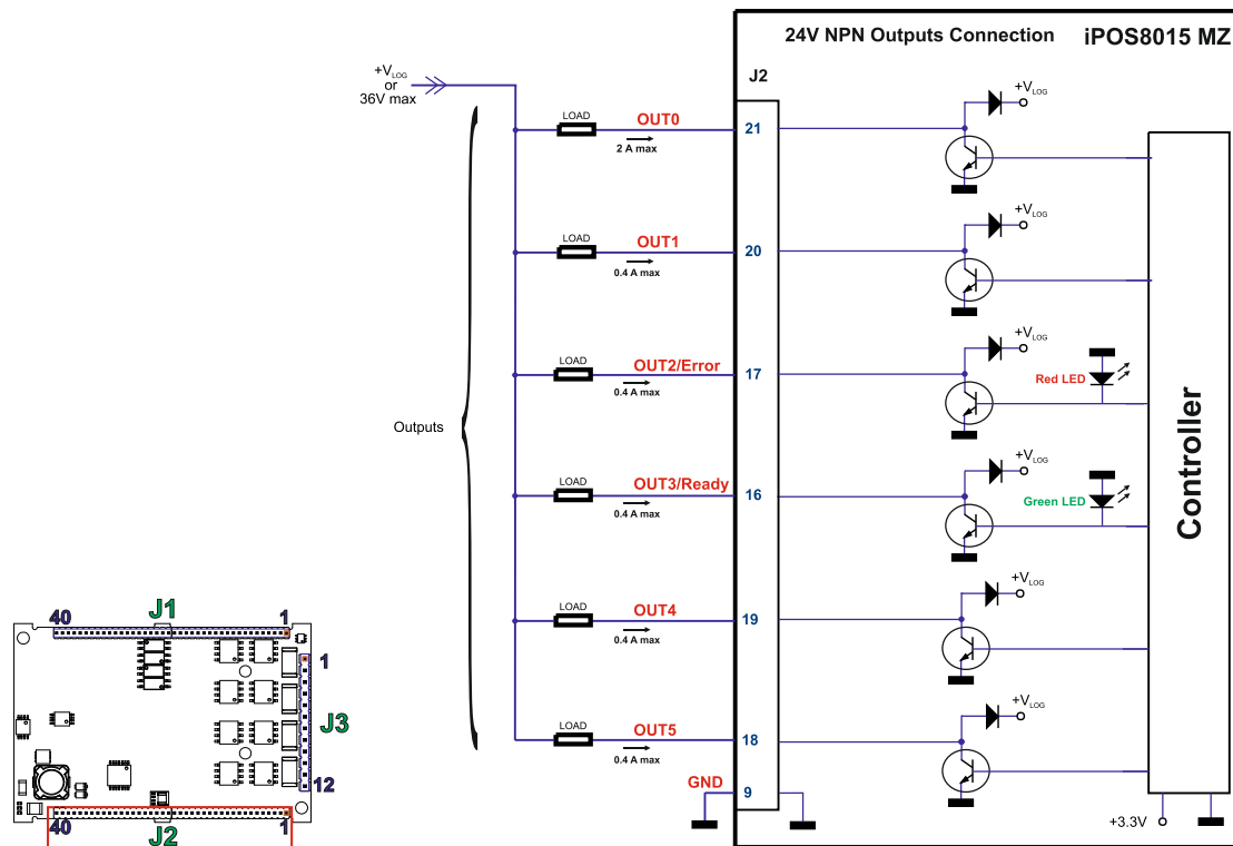
Figure 13.6. 24V Digital NPN Outputs connection
