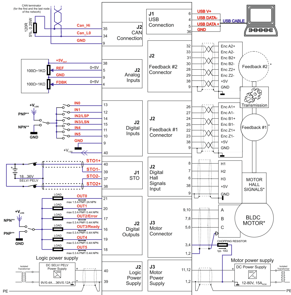
Figure 13.2. iPOS8015 MZ-CAN Connection diagram
