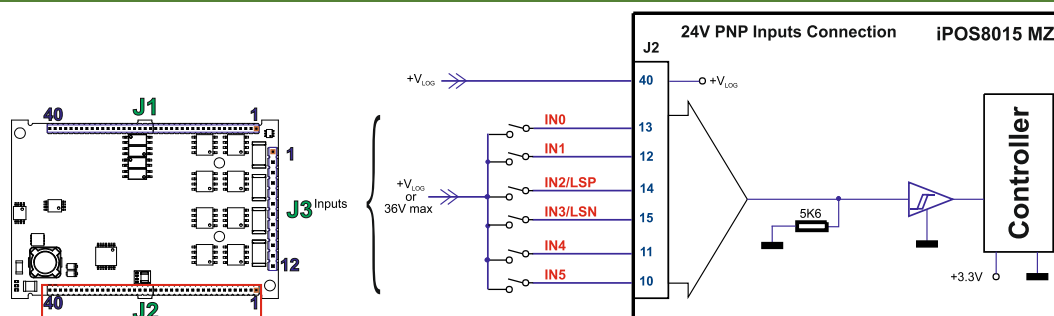
Figure 13.3. 24V Digital PNP Inputs connection
