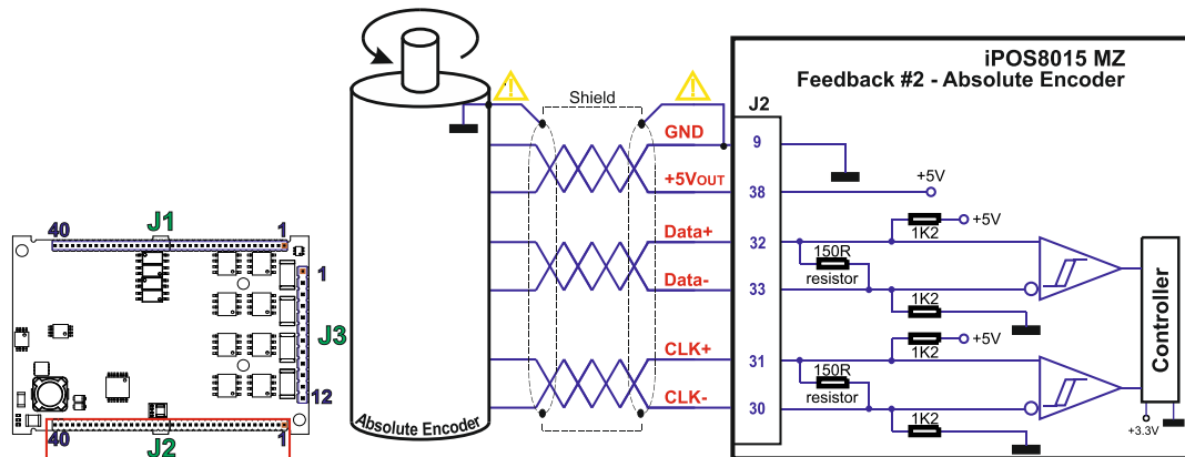
Figure 13.21. Feedback #2 – Absolute Encoder Connection: SSI, BiSS, EnDAT
