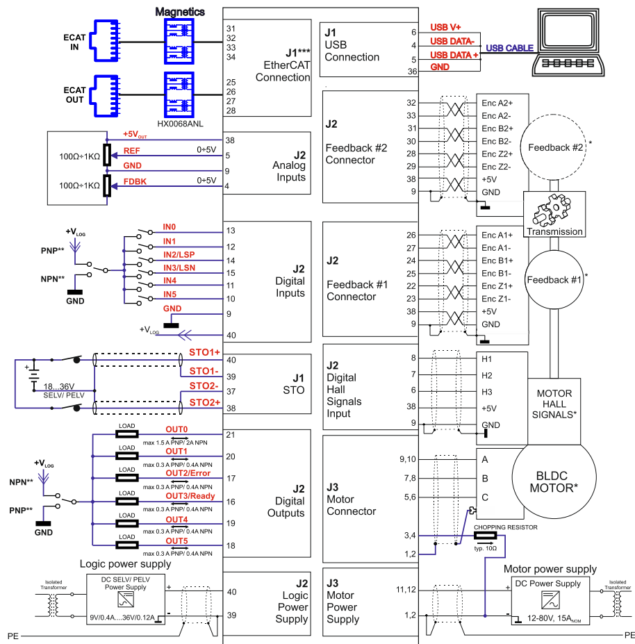
Figure 13.1. iPOS8015 MZ-CAT Connection diagram
