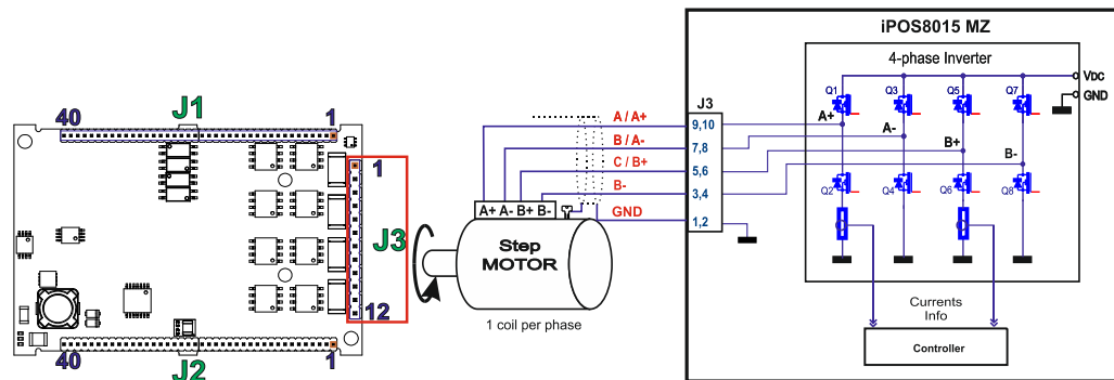
Figure 13.13. 2-phase step motor connection, one coil per phase
