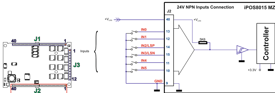
Figure 13.4. 24V Digital NPN Inputs connection
