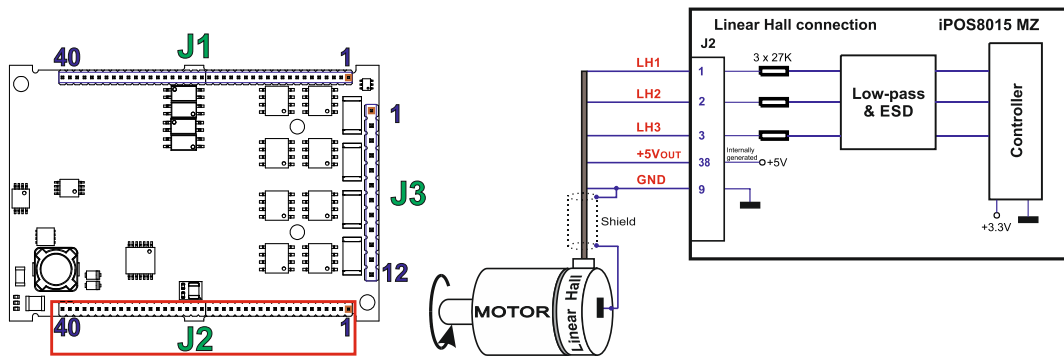
Figure 13.23. Linear Hall connection
