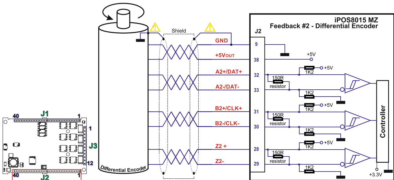
Figure 13.19. Differential incremental encoder #2 connection
