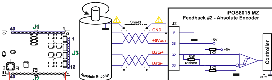
Figure 13.22. Feedback #2 – Absolute Encoder Connection: Panasonic, Tamagawa, Nikon, Sanyo Denki
