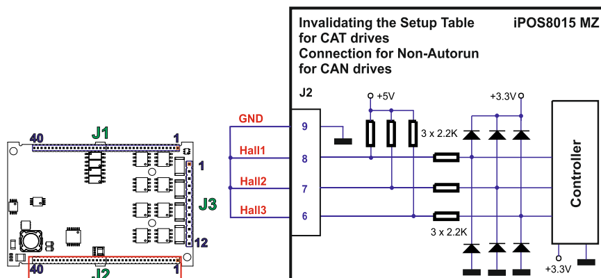
Figure 13.33. Temporary connection during power-on to remove the drive from Autorun mode or invalidate the Setup table
