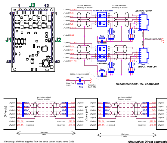
Figure 13.32. EtherCAT bus to RJ45 connection PoE compliant
