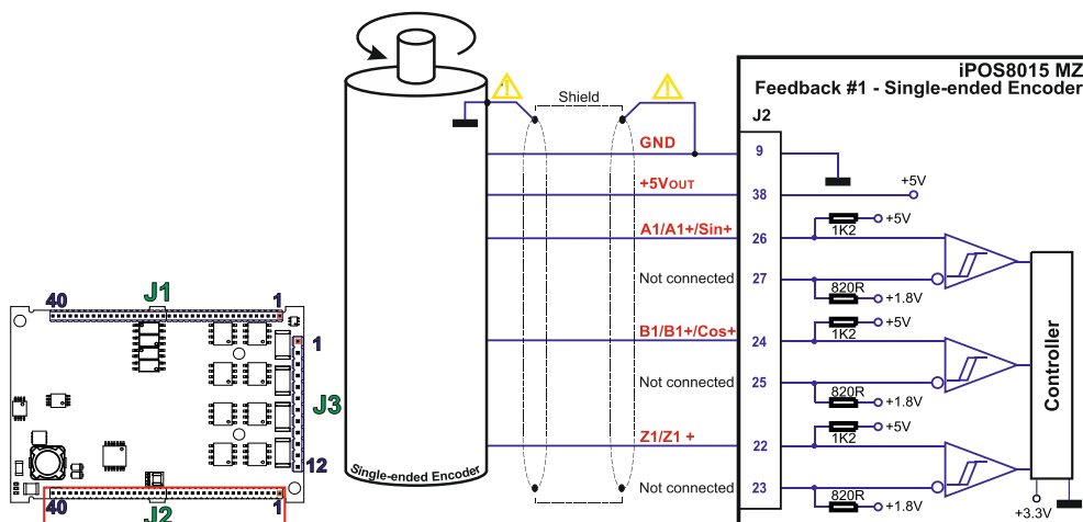
Figure 13.17. Single-ended incremental encoder connection
