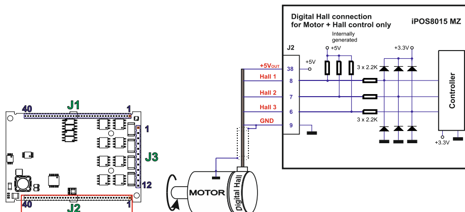
Figure 13.25. Digital Hall connection
