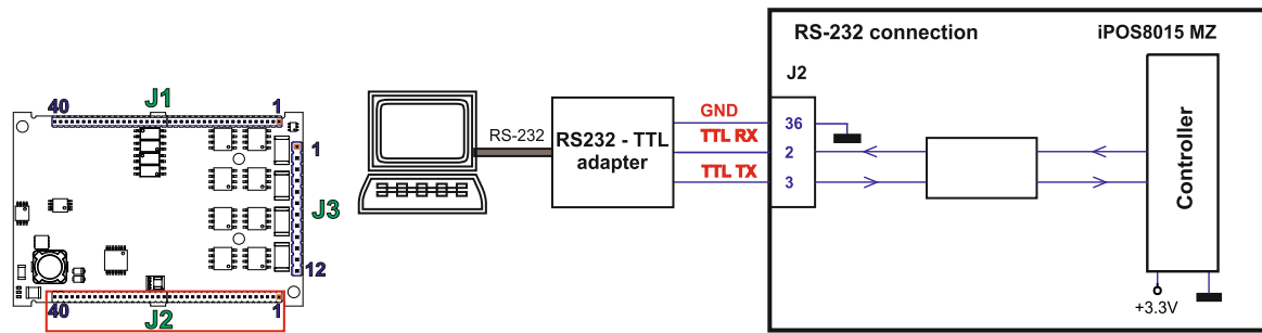
Figure 13.28. Low level TTL connection
