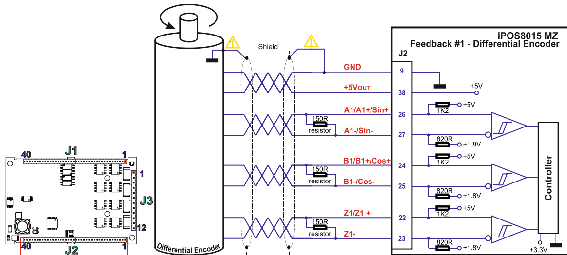
Figure 13.18. Differential incremental encoder #1 connection
