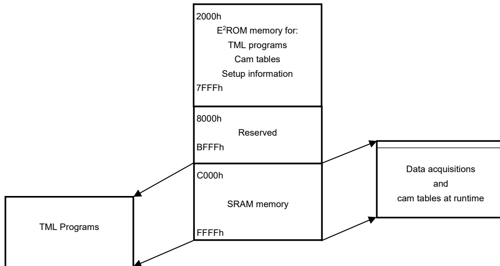
Figure 14.1 iPOS8015 MZ Memory Map
