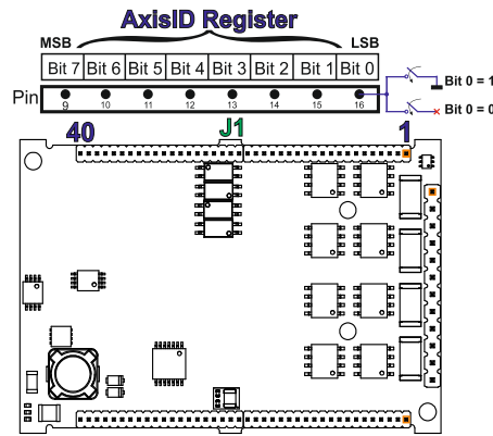
Figure 13.35. J1 – Axis ID pins for CAT drives
