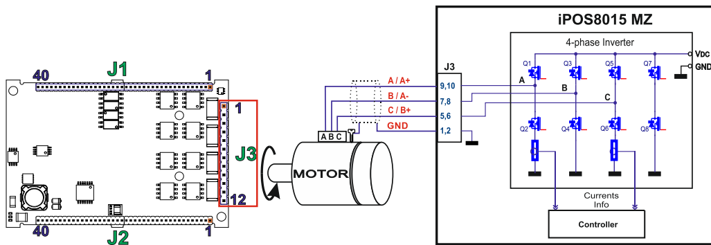
Figure 13.12. Brushless motor connection
