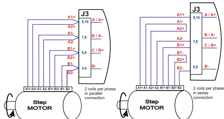
Figure 13.14. 2-phase step motor connection, two coils per phase
