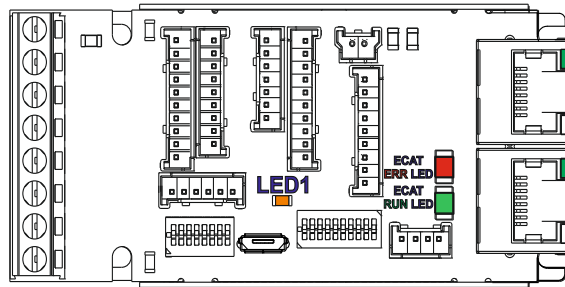
Figure 41. LED indicators
