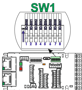
Figure 40. SW1 – DIP Switch settings
