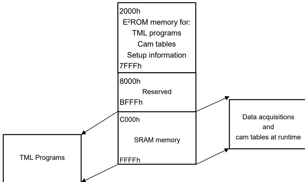
Figure 43. iPOS481x XZ Memory Map
