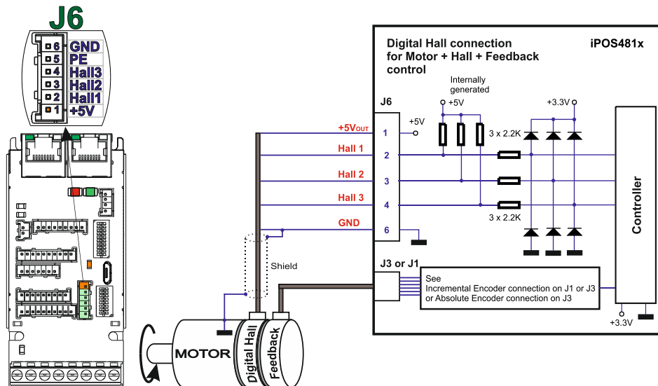
Figure 26. Digital Hall connection for Motor + Hall +Feedback control
