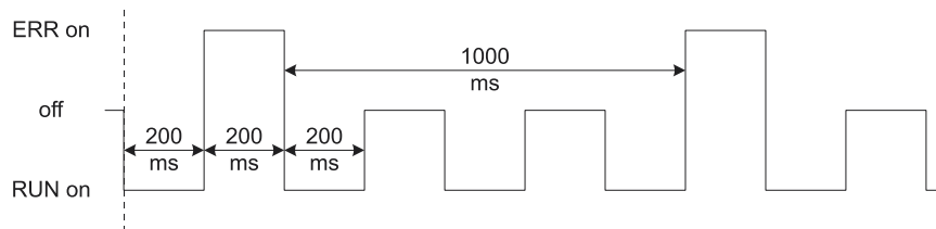
Figure 42. STATUS indicator Example
