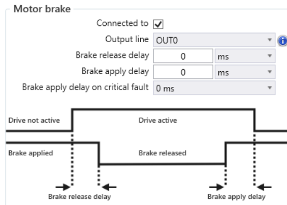
Figure 11. Motor brake checkbox in EasyMotion Studio II
