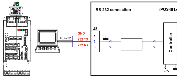
Figure 3.32. Low level TTL connection
