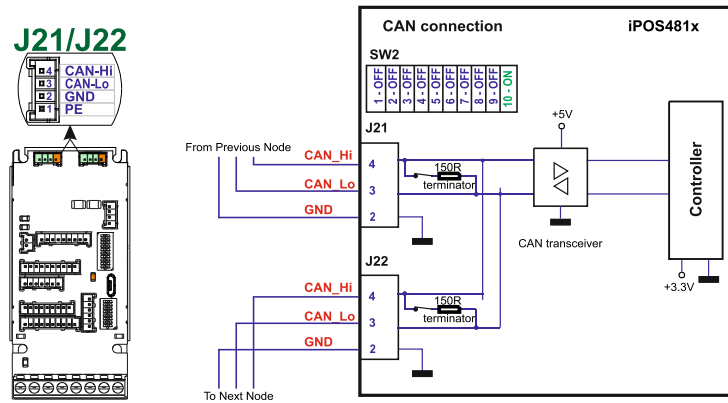
Figure 33. CAN connection
