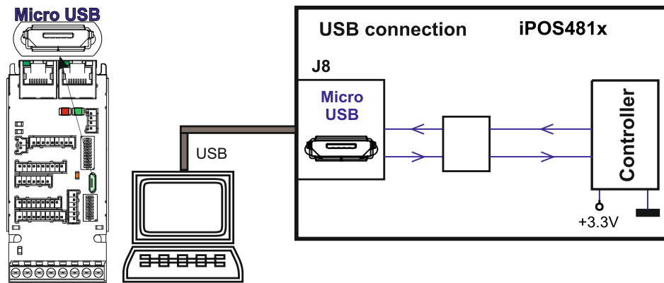
Figure 31. USB connection
