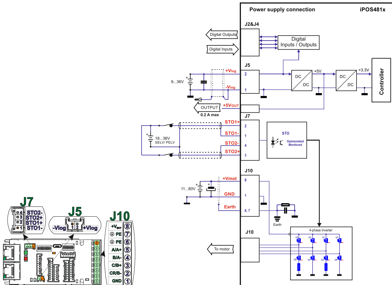
Figure 29. Supply connection
