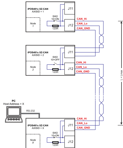
Figure 34. Multiple-Axis CAN network
