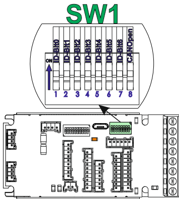
Figure 38. SW1 – DIP Switch settings
