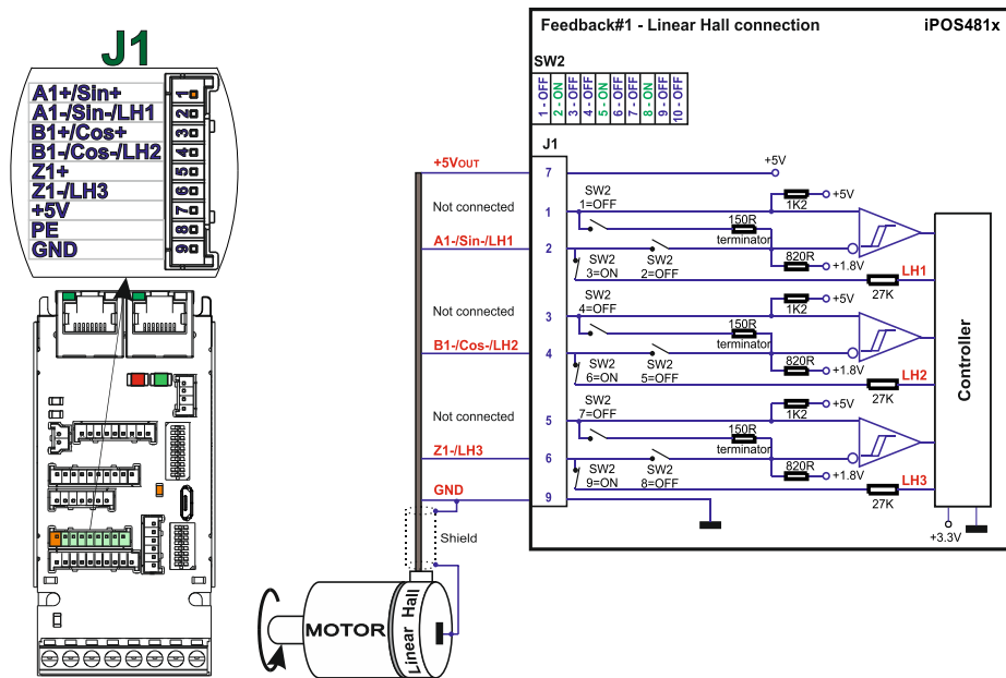
Figure 24. Linear Hall connection
