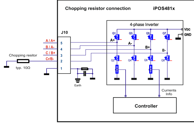
Figure 30. Chopping resistor connection
