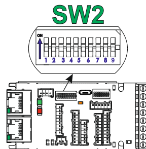
Figure 25. SW2 DIP Switch
