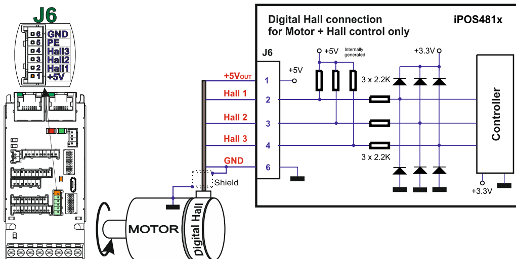
Figure 27. Digital Hall connection for Motor + Hall control
