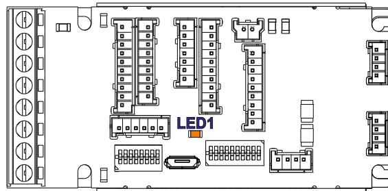
Figure 39. LED indicators
