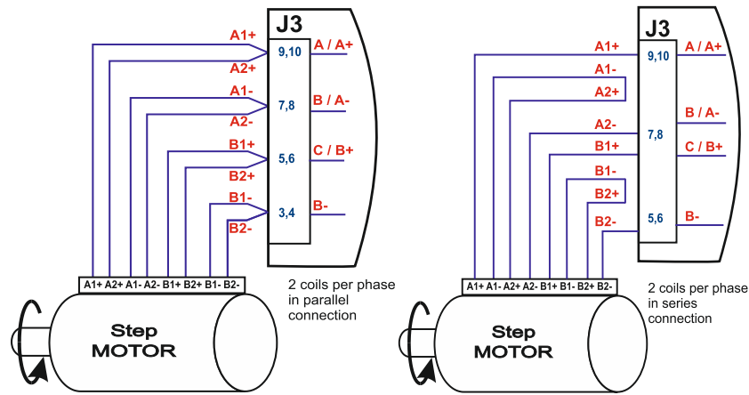
Figure 2.14. 2-phase step motor connection, two coils per phase
