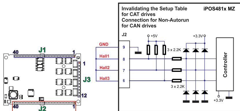
Figure 2.33. Temporary connection during power-on to remove the drive from Autorun mode or invalidate the Setup table
