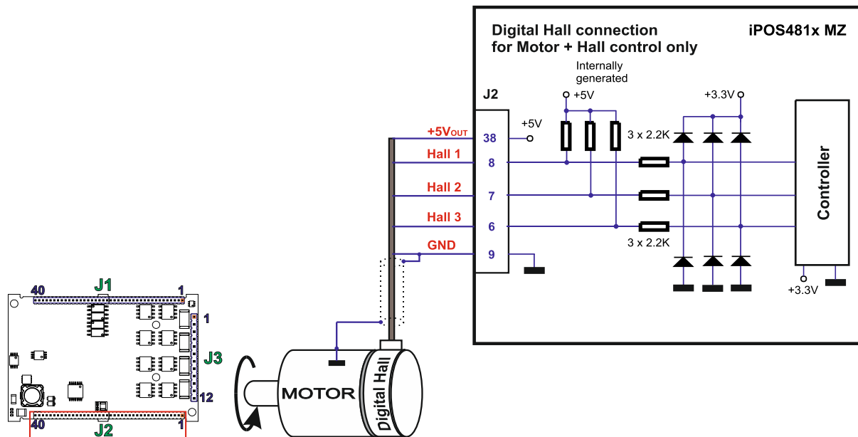
Figure 2.25. Digital Hall connection
