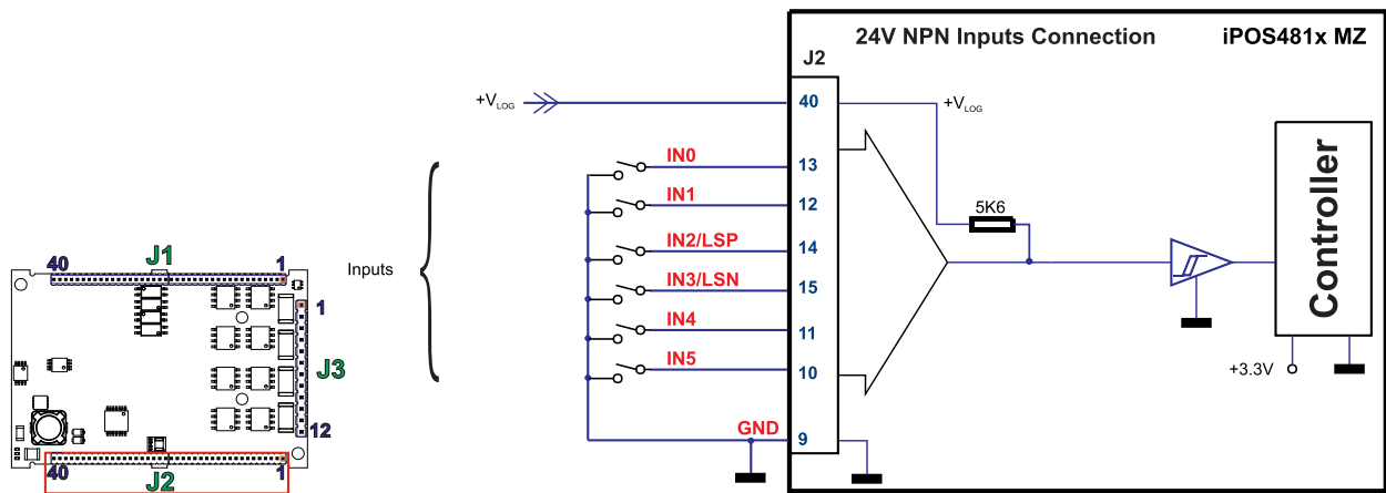
Figure 2.4. 24V Digital NPN Inputs connection
