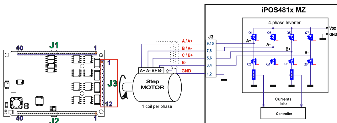
Figure 2.13. 2-phase step motor connection, one coil per phase
