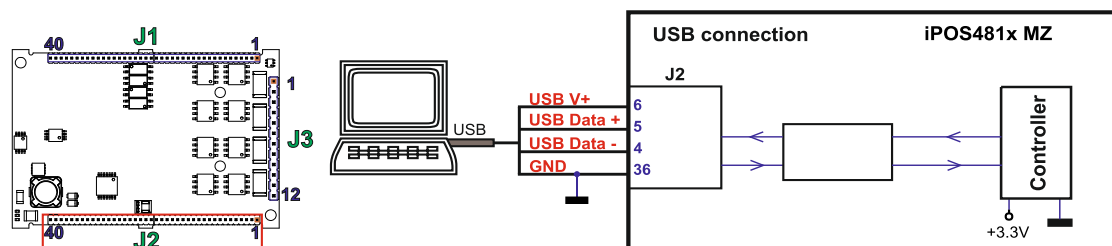
Figure 2.29. USB connection
