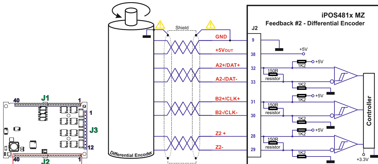
Figure 2.19. Differential incremental encoder #2 connection
