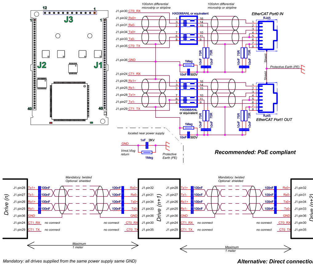
Figure 2.32. EtherCAT bus to RJ45 connection PoE compliant
