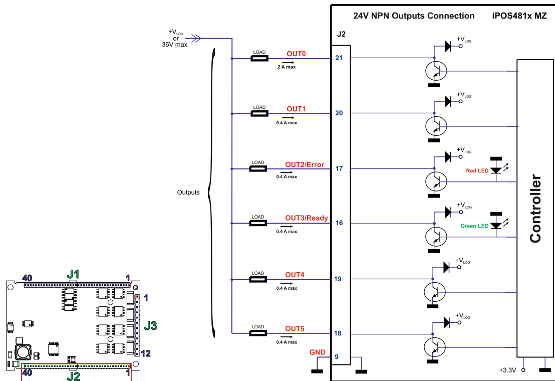
Figure 2.6. 24V Digital NPN Outputs connection
