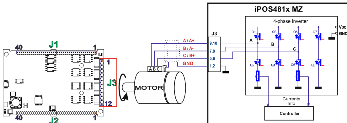
Figure 2.12. Brushless motor connection
