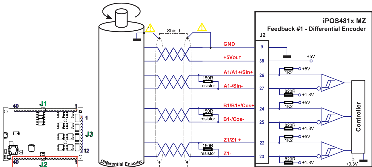
Figure 2.18. Differential incremental encoder #1 connection
