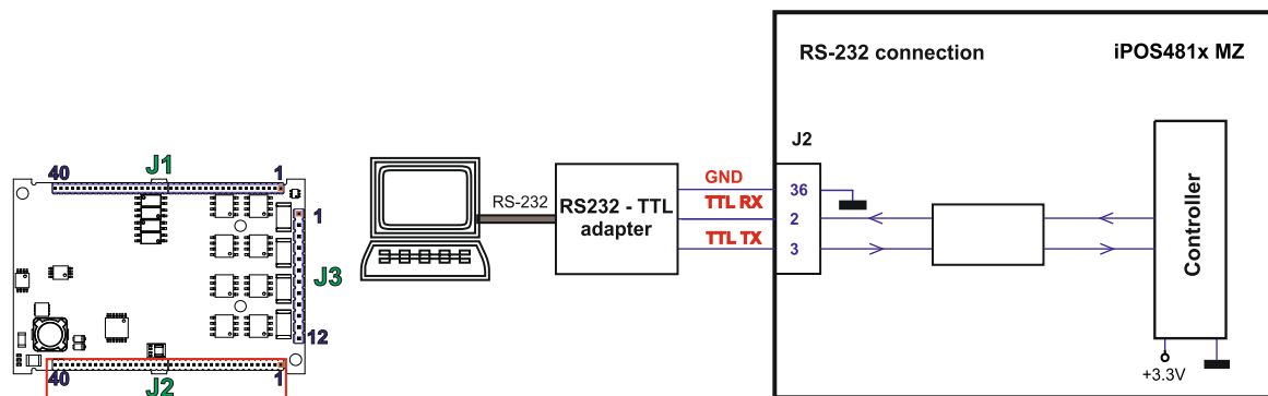
Figure 2.28. Low level TTL connection
