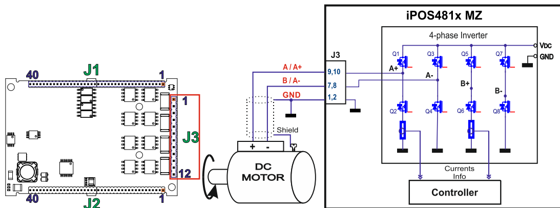
Figure 2.16. DC Motor connection
