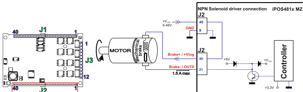
Figure 10 Solenoid driver connection
