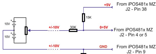
Figure 2.9. +/-10V to 0-5V adapter
