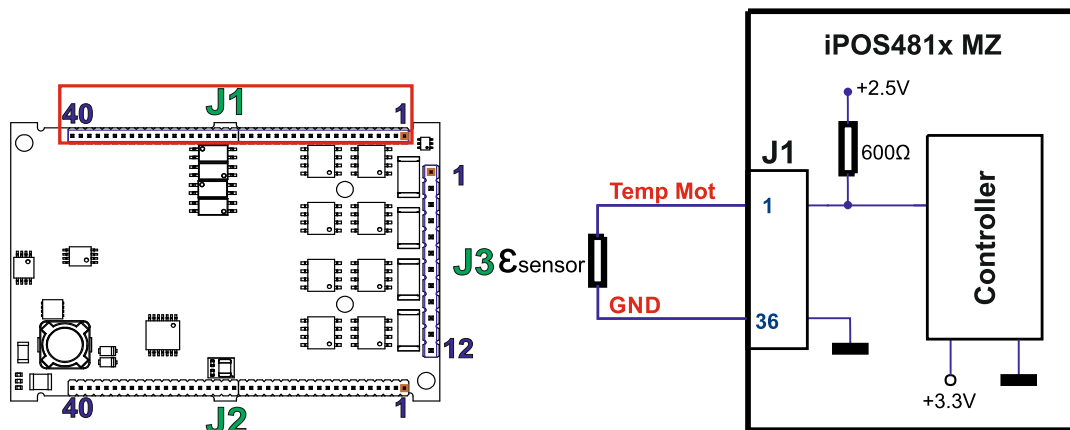
Figure 2.7. Temperature sensor connection
