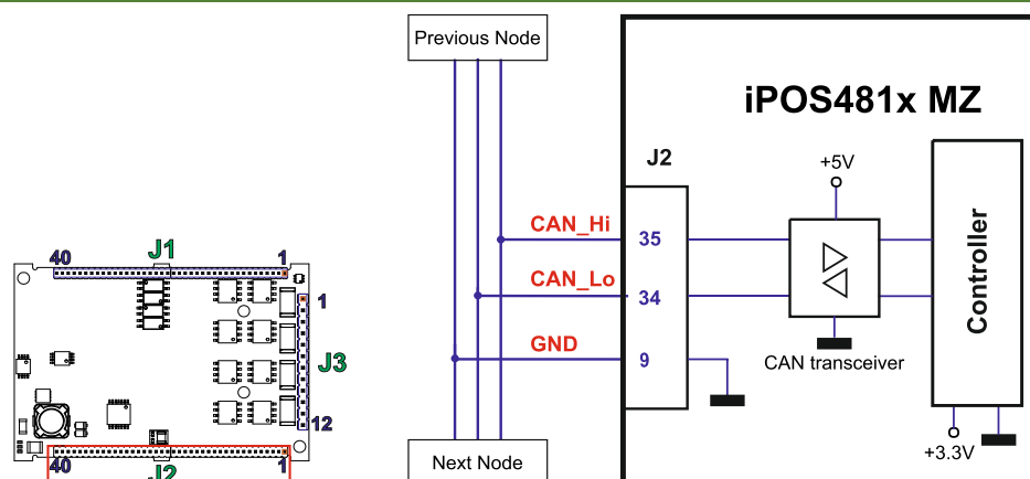
Figure 2.30. CAN connection
