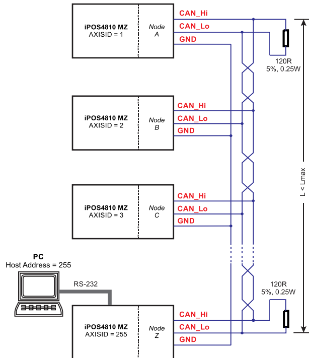
Figure 2.31. Multiple-Axis CAN network
