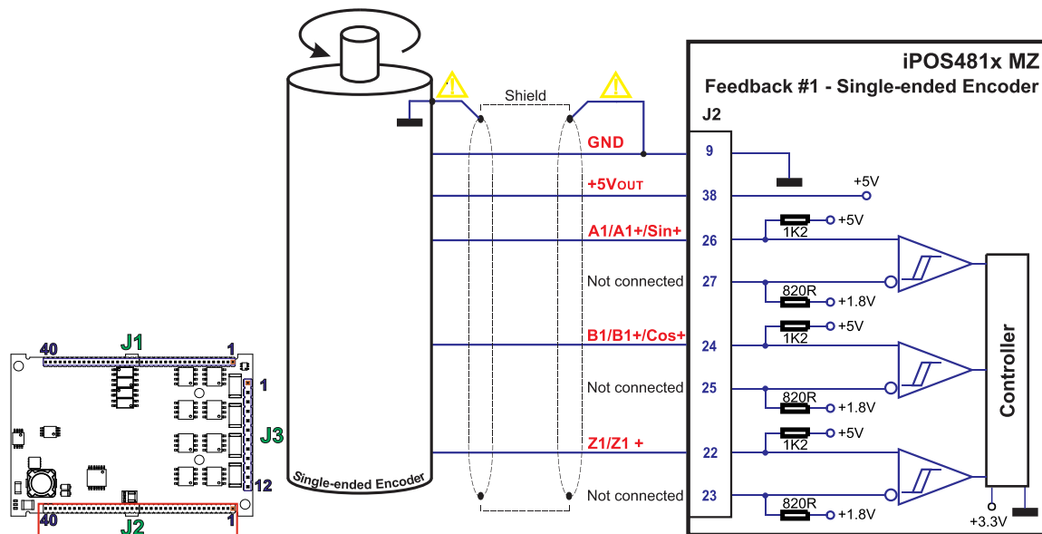
Figure 2.17. Single-ended incremental encoder connection
