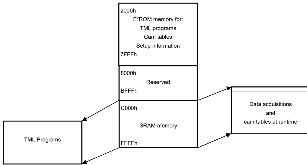
Figure 4.1. iPOS481x MZ Memory Map
