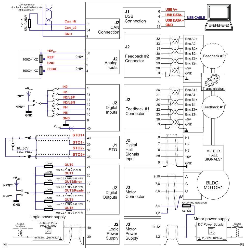
Figure 2.2. iPOS481x MZ-CAN Connection diagram
