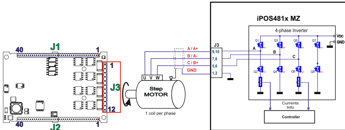
Figure 2.15. 3-phase step motor connection
