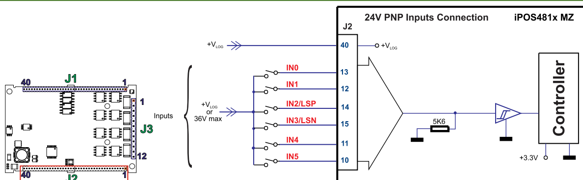
Figure 2.3. 24V Digital PNP Inputs connection
