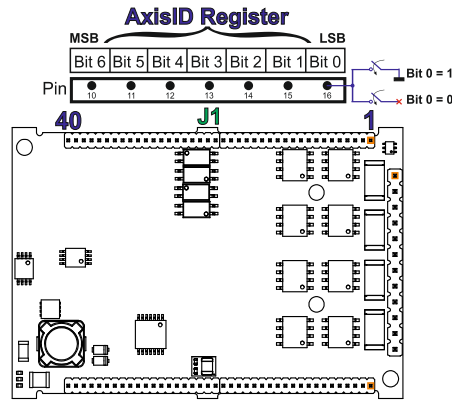
Figure 2.34. J1 – Axis ID pins for CAN drives
