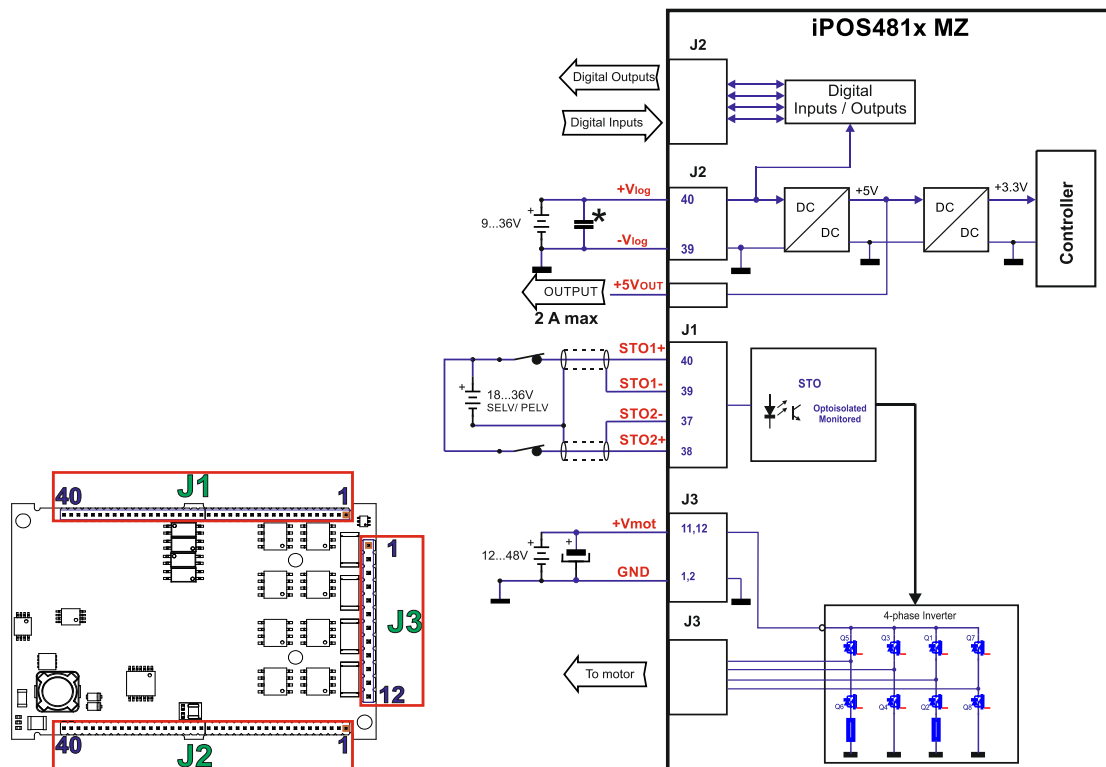
Figure 2.26. Supply connection
