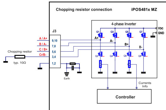
Figure 2.27. Chopping resistor connection
