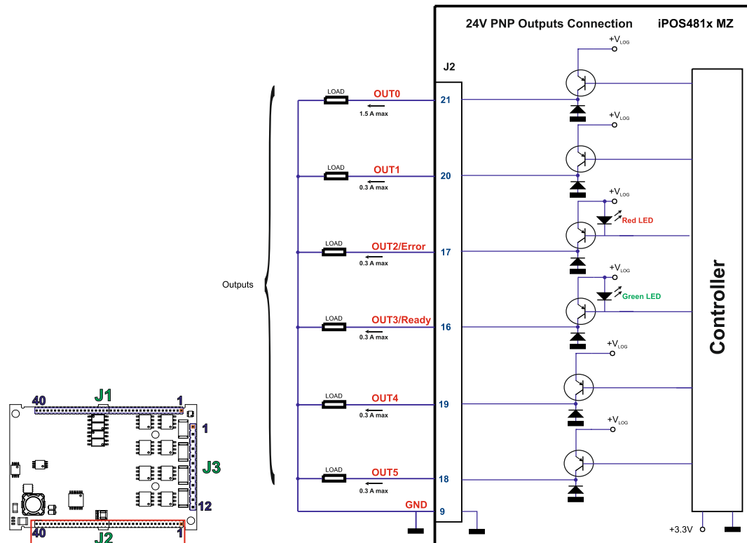
Figure 2.5. 24V Digital PNP Outputs connection
