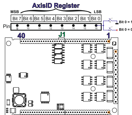
Figure 2.35. J1 – Axis ID pins for CAT drives
