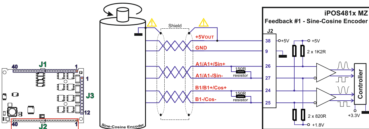
Figure 2.20. Sine-Cosine analogue encoder connection
