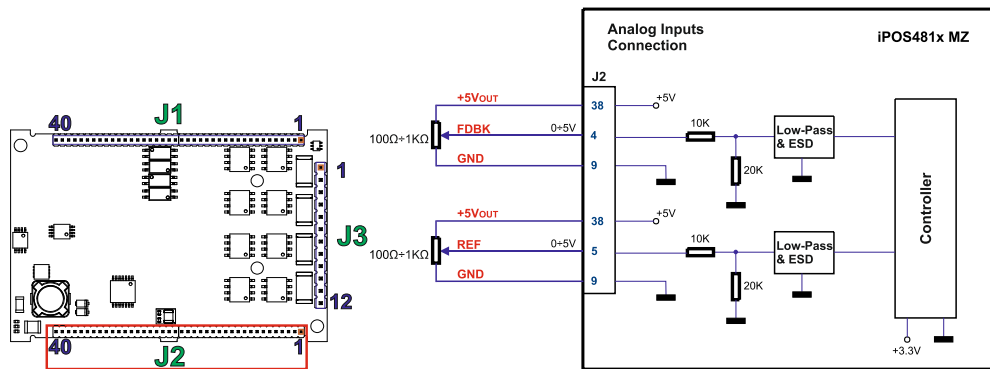
Figure 2.8. 0-5V Analog inputs connection
