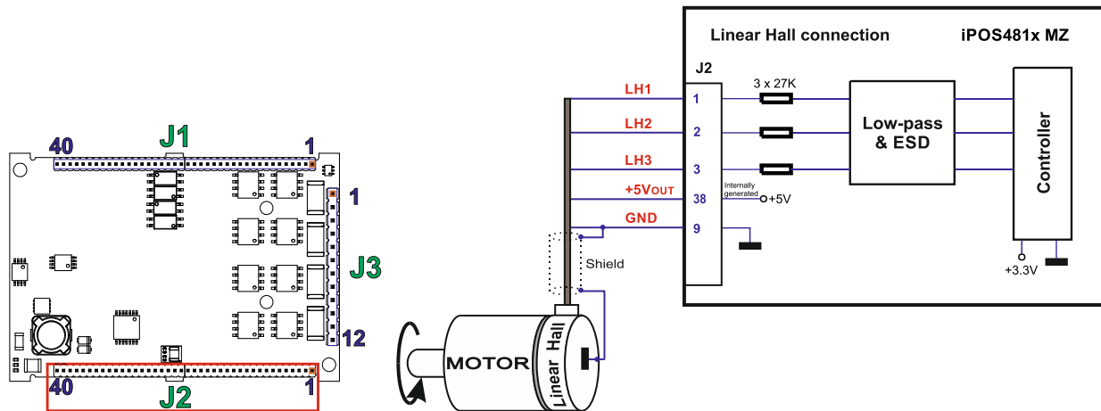
Figure 2.23. Linear Hall connection
