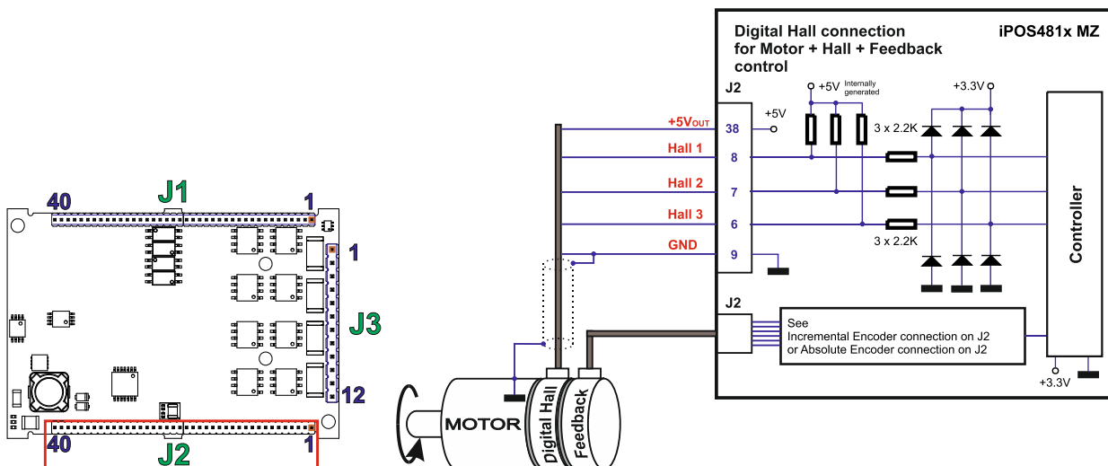
Figure 2.24. Digital Hall connection
