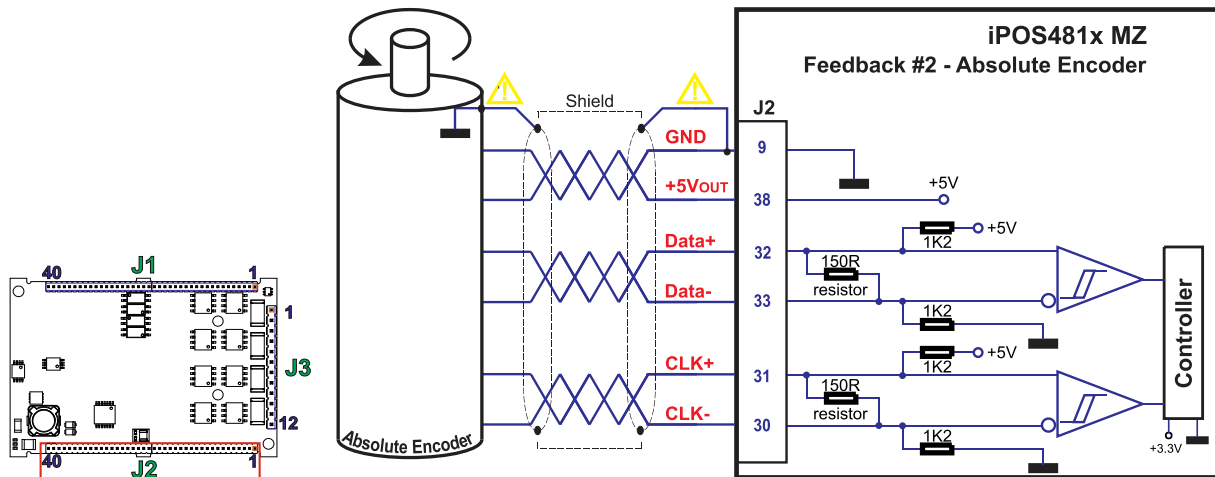
Figure 2.21. Feedback #2 – Absolute Encoder Connection: SSI, BiSS, EnDAT
