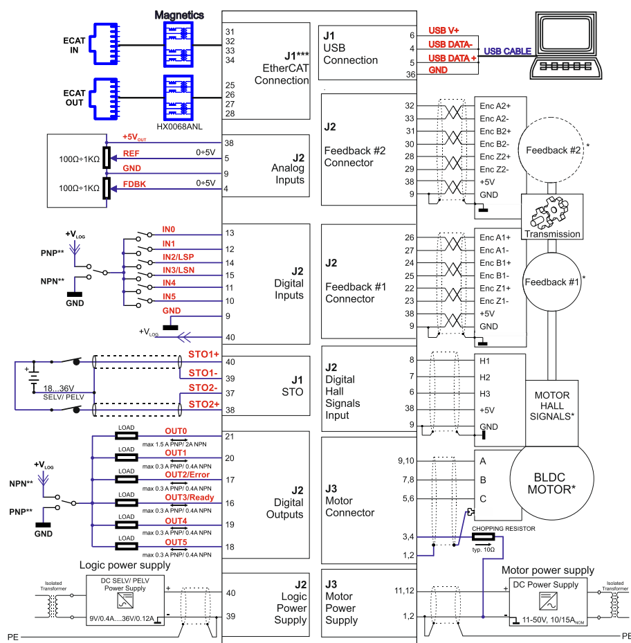
Figure 2.1. iPOS481x MZ-CAT Connection diagram
