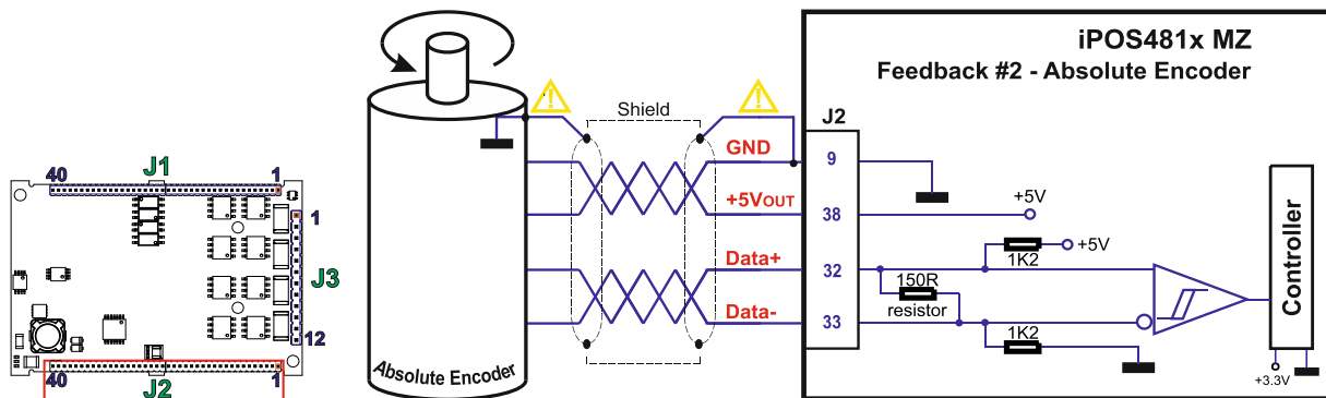
Figure 2.22. Feedback #2 – Absolute Encoder Connection: Panasonic, Tamagawa, Nikon, Sanyo Denki
