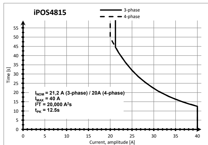
iPOS4815 – Over-current diagram (No heatsink)
