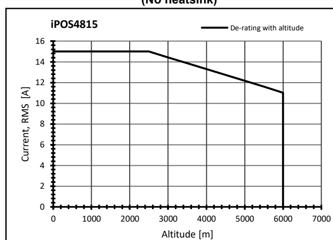
iPOS4815 – De-rating with the altitude
