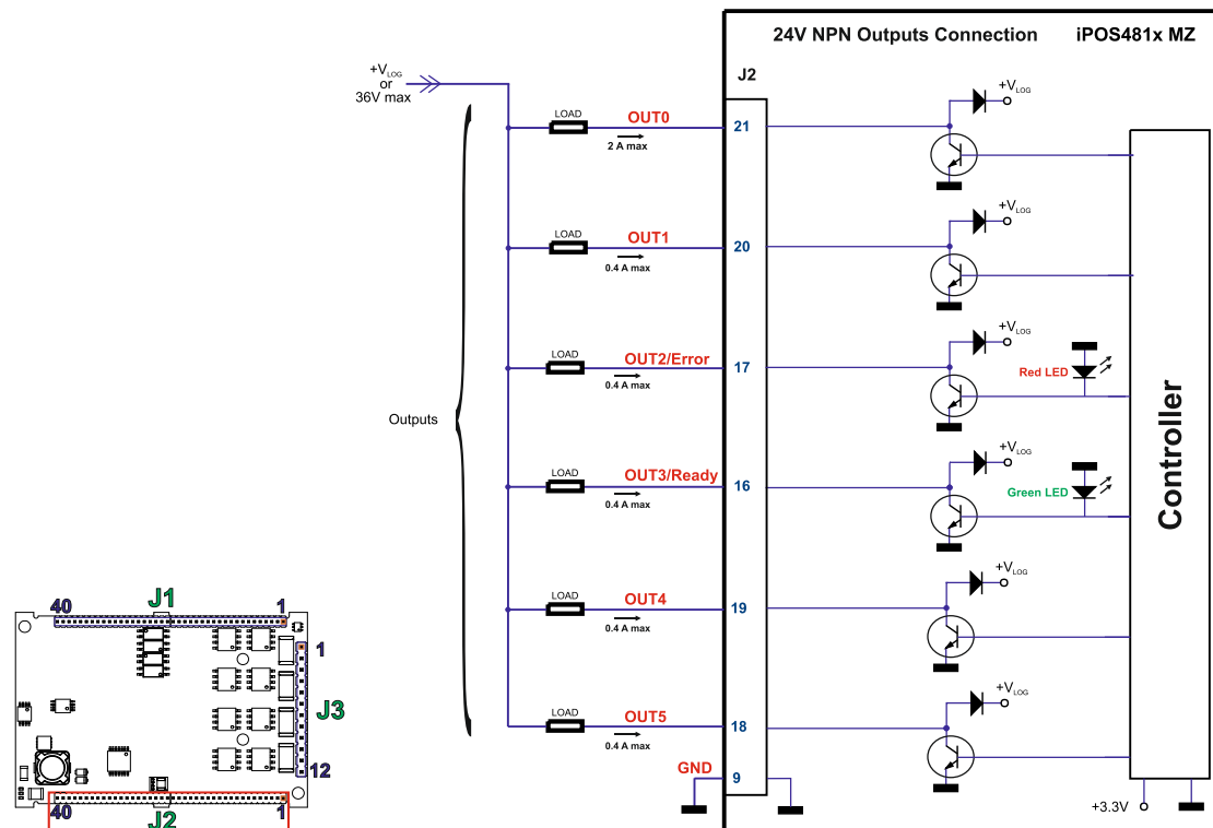
Figure 2.6. 24V Digital NPN Outputs connection
