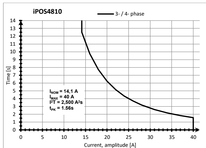
iPOS4810 – Over-current diagram (No heatsink)
