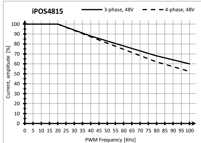
iPOS4815 – Current de-rating with PWM frequency
