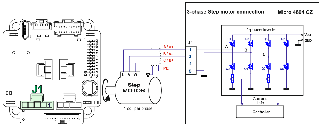
Figure 3-36 3-phase step motor connection for Micro 4804 CZ
