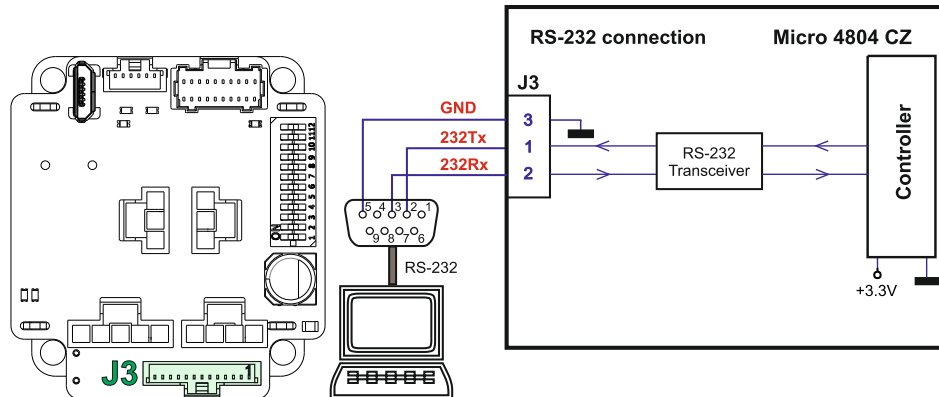
Figure 3-68. Serial RS-232 connection for Micro 4804 CZ
