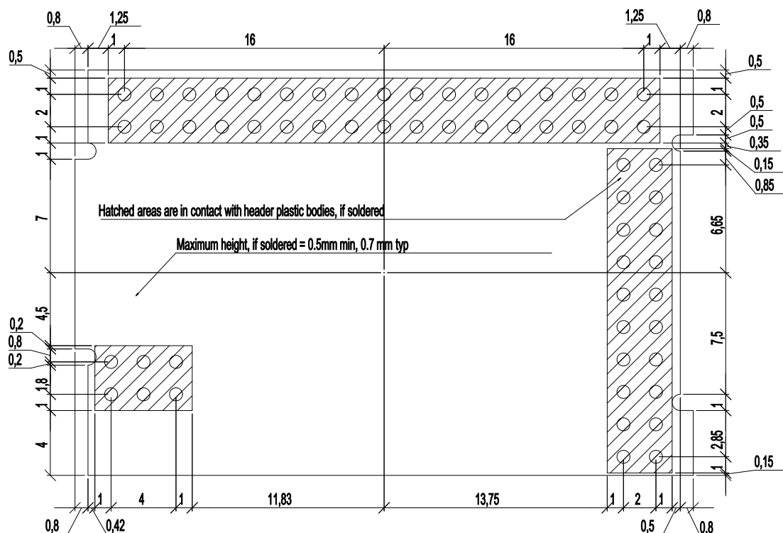
Figure 3-9 Micro MZ and LZ PCB Footprint – Pins facing downward view
