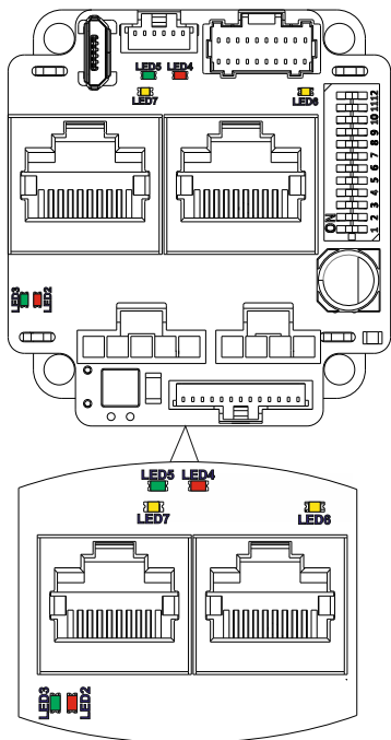
Figure 3-79 LED indicators for Micro 4804 CZ
