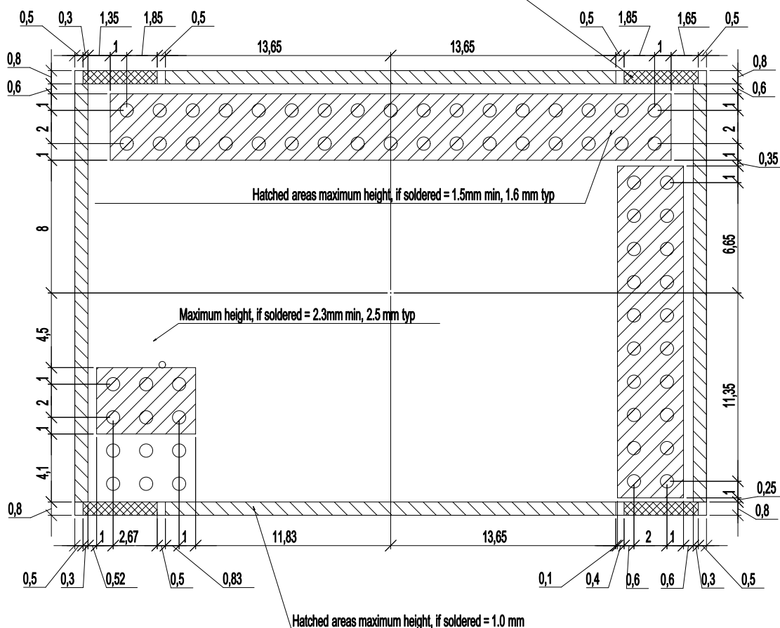
Figure 3-11 Micro 4804 PZ PCB Footprint – Pins facing upward view
