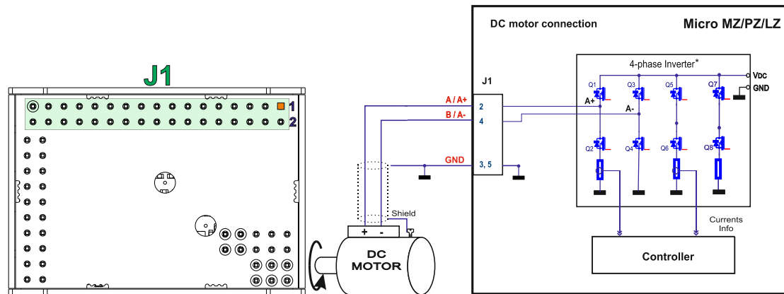
Figure 3-37 DC Motor connection for Micro MZ/PZ/LZ
