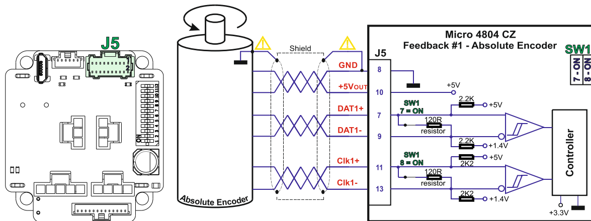
Figure 3-48 Feedback #1 – Absolute Encoder Connection for Micro 4804 CZ
