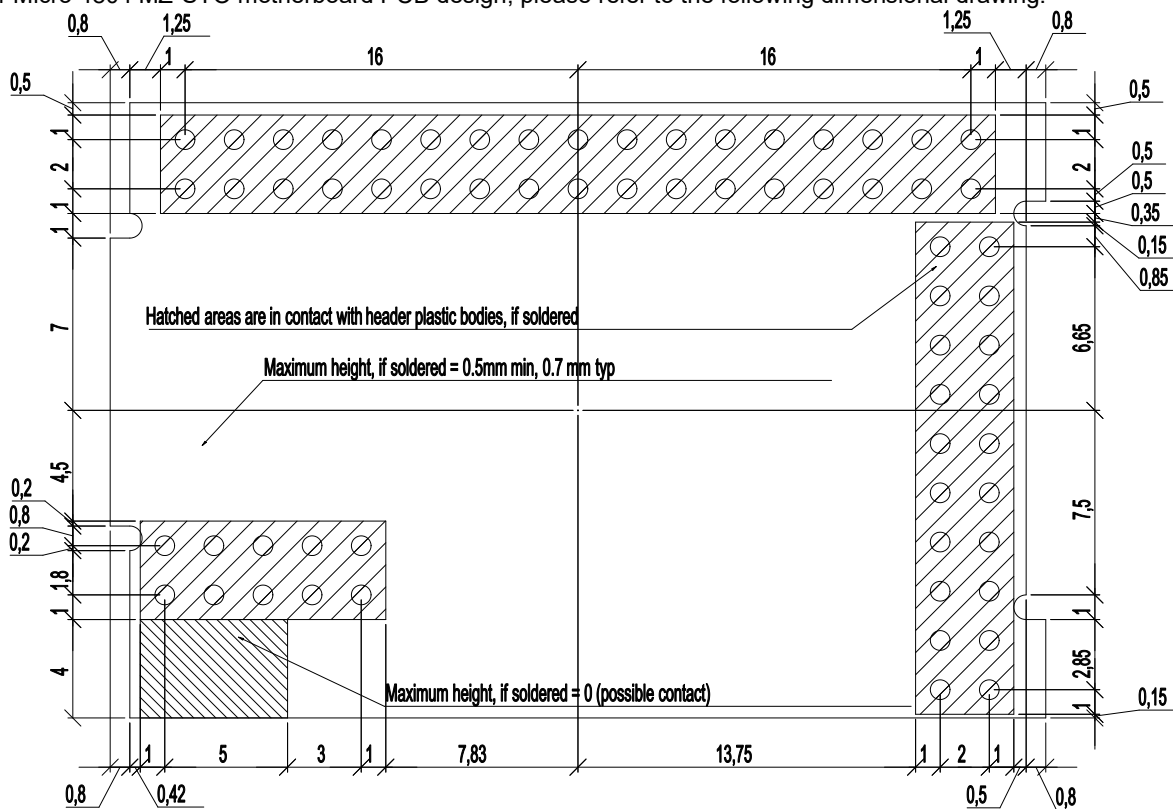
Figure 3-10 Micro 4804 MZ-STO PCB Footprint – Pins facing downward view
