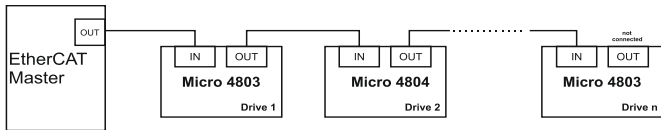
Figure 3-72 EtherCAT network linear topology
