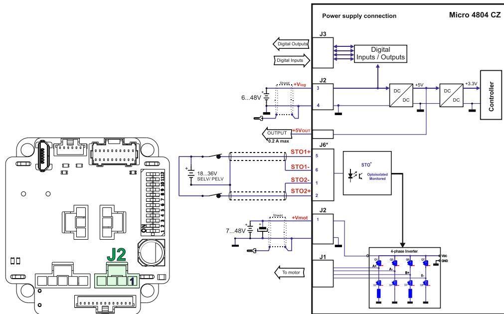
Figure 3-62 Supply connection for Micro 4804 CZ
