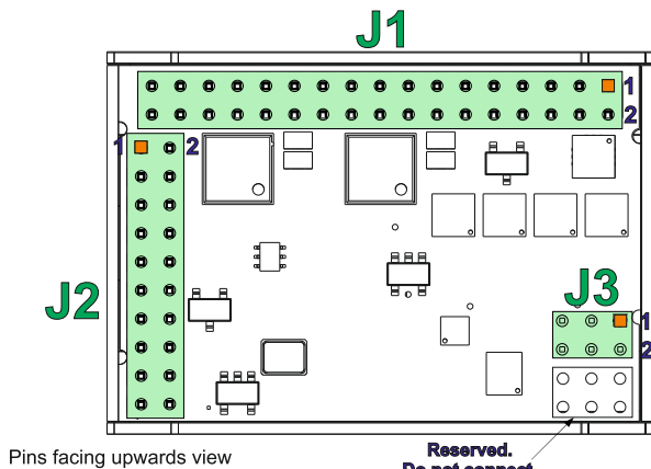
Pins facing upwards view
