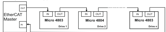
Figure 3-73 EtherCAT network ring topology
