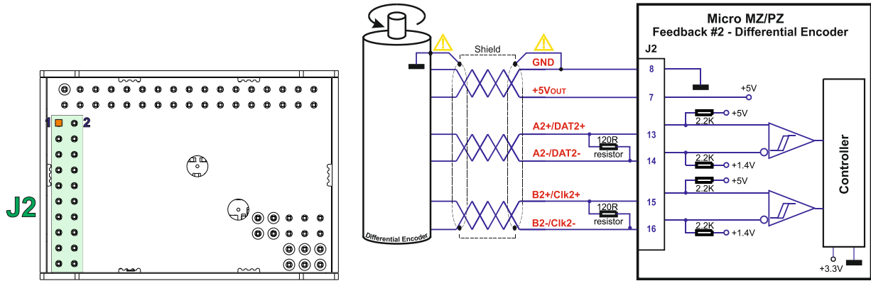
Figure 3-45 Feedback #2 - Differential Incremental Encoder Connection for Micro MZ/PZ
