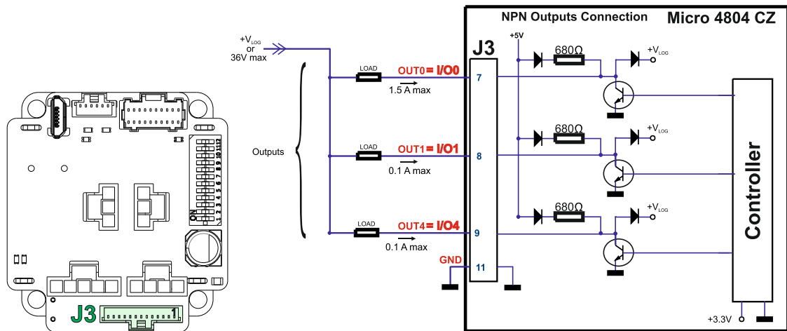
Figure 3-21 Digital NPN Outputs connection for Micro 4804 CZ
