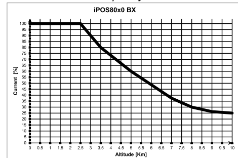
iPOS8020 BX-CAT De-rating with altitude
