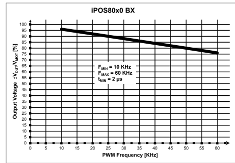
iPOS8020 BX-CAT Output Voltage De-rating with PWM frequency 1
