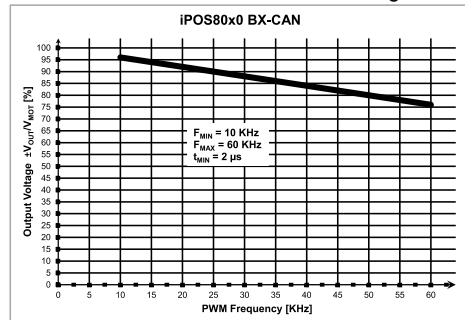
iPOS8020 BX-CAN Output Voltage De-rating with PWM frequency 1
