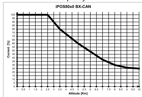
iPOS8020 BX-CAN De-rating with altitude
