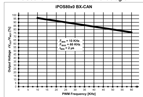
iPOS8010 BX-CAN Output Voltage De-rating with PWM frequency 1
