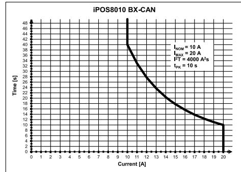
iPOS8010 BX-CAN Over-current diagram
