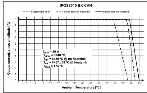
iPOS8010 BX-CAN De-rating with ambient temperature
