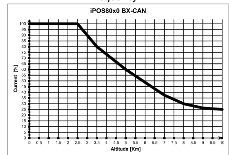
iPOS8010 BX-CAN De-rating with altitude
