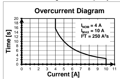
Over-current diagram
