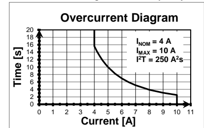
Over-current diagram
