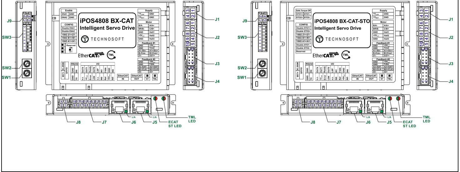
iPOS4808 BX-CAT and iPOS4808 BX-CAT-STO connectors and pinout
