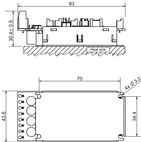
All dimensions are in mm; Drawing not to scale.
