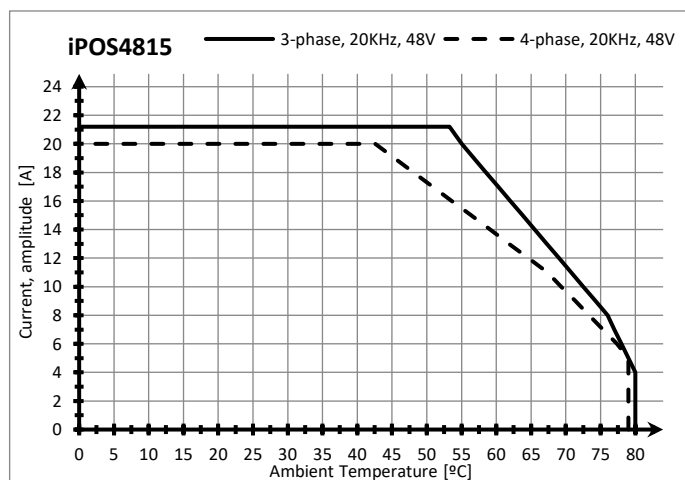
iPOS4815 MZ – Current de-rating with ambient temperature
