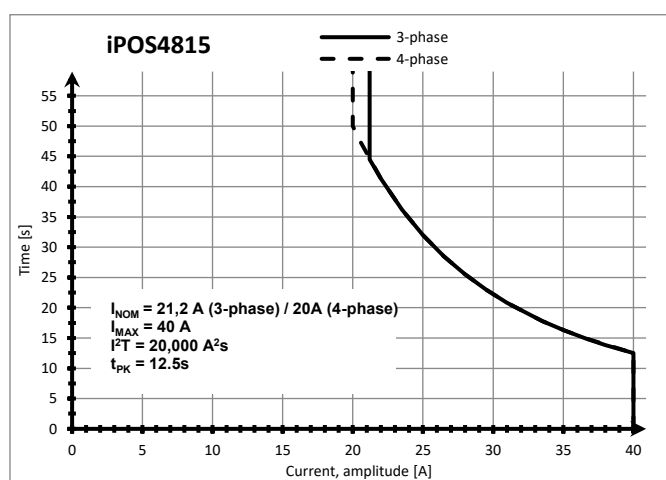
iPOS4815 MZ – Over-current diagram (No heatsink)
