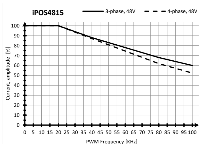
iPOS4815 MZ – Current de-rating with PWM frequency
