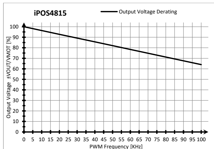
iPOS4815 MZ – Output Voltage de-rating with PWM frequency
