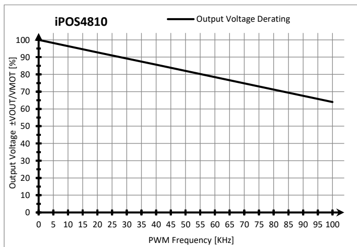
iPOS4810 MZ – Output Voltage de-rating with PWM frequency
