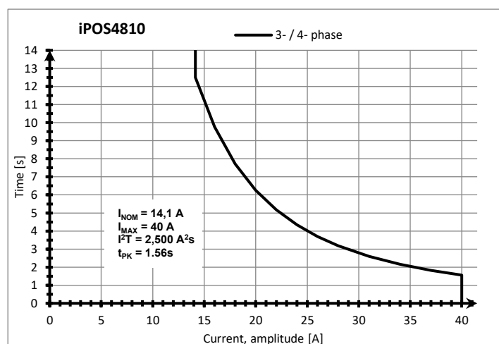
iPOS4810 MZ – Over-current diagram (No heatsink)
