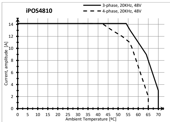
iPOS4810 MZ – Current de-rating with ambient temperature
