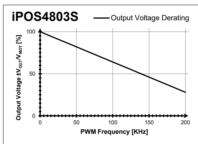
Figure 4 iPOS4803S Output Voltage De-rating with PWM frequency
