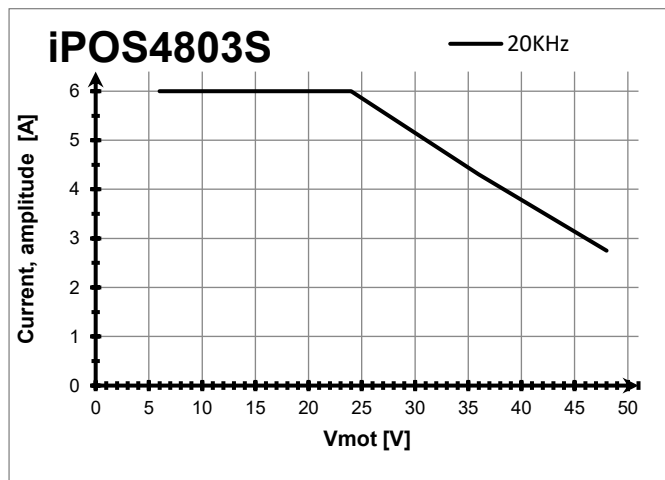
Figure 3 iPOS4803S De-rating with motor supply
