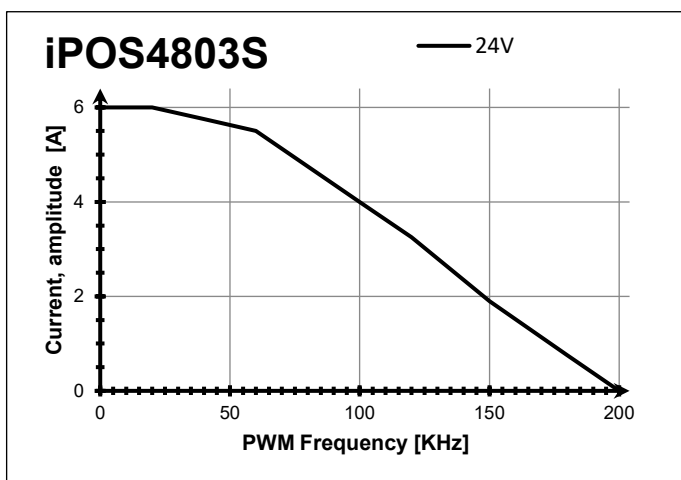
Figure 1 iPOS4803S De-rating with PWM frequency
