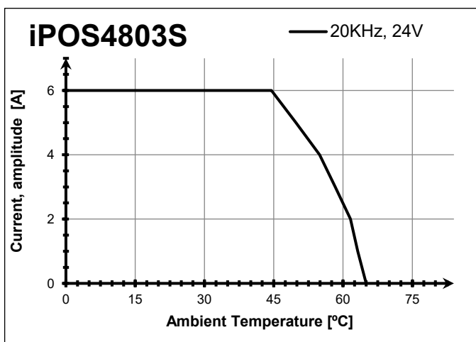
Figure 2 iPOS4803S De-rating with ambient temperature
